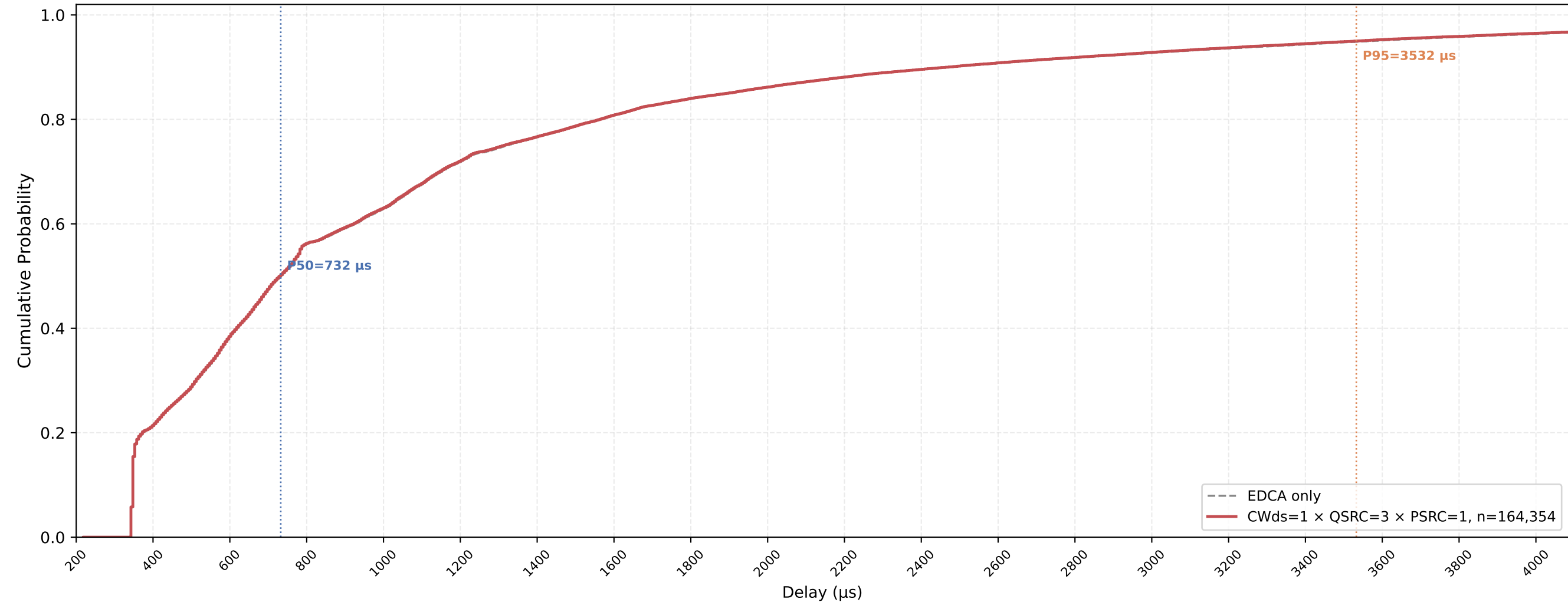
VO (all STAs) Delay CDF — CWds=1 × QSRC=3 × PSRC=1 nSta=30, nPedca=5, 0.5Mbps, avg of 10 runs
