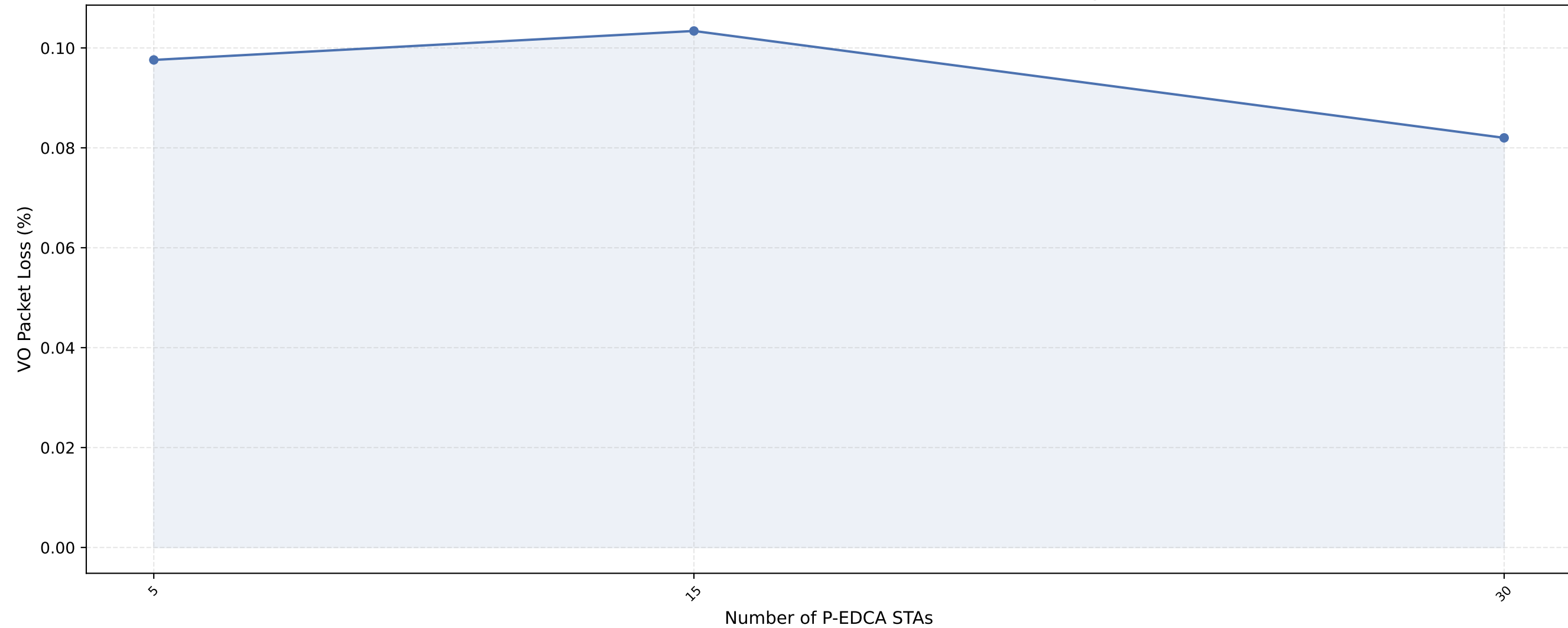
VO Packet Loss vs P-EDCA STAs — nSta=30, 0.5Mbps (avg of 10 runs)
