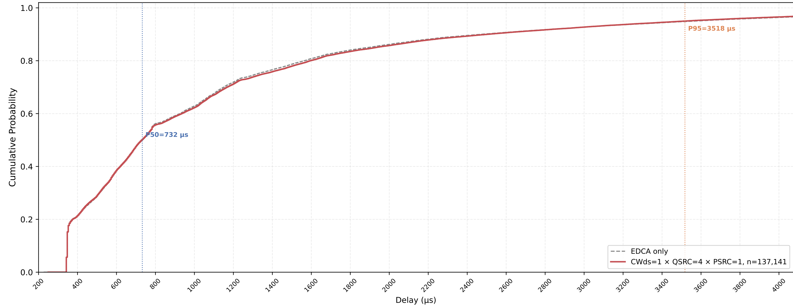
Legacy STA VO Delay CDF — CWds=1 × QSRC=4 × PSRC=1 nSta=30, nPedca=5, 0.5Mbps, avg of 10 runs
