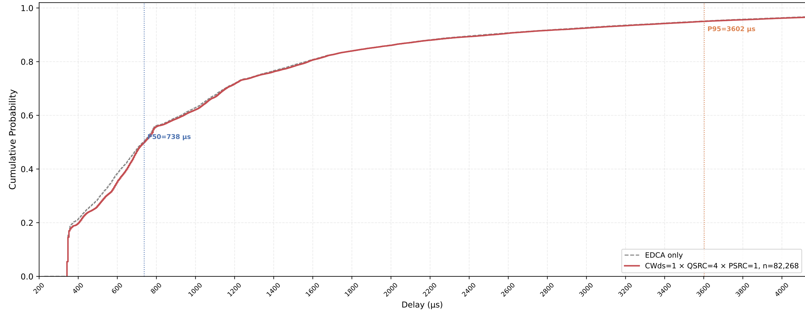
Legacy STA VO Delay CDF — CWds=1 × QSRC=4 × PSRC=1 nSta=30, nPedca=15, 0.5Mbps, avg of 10 runs
