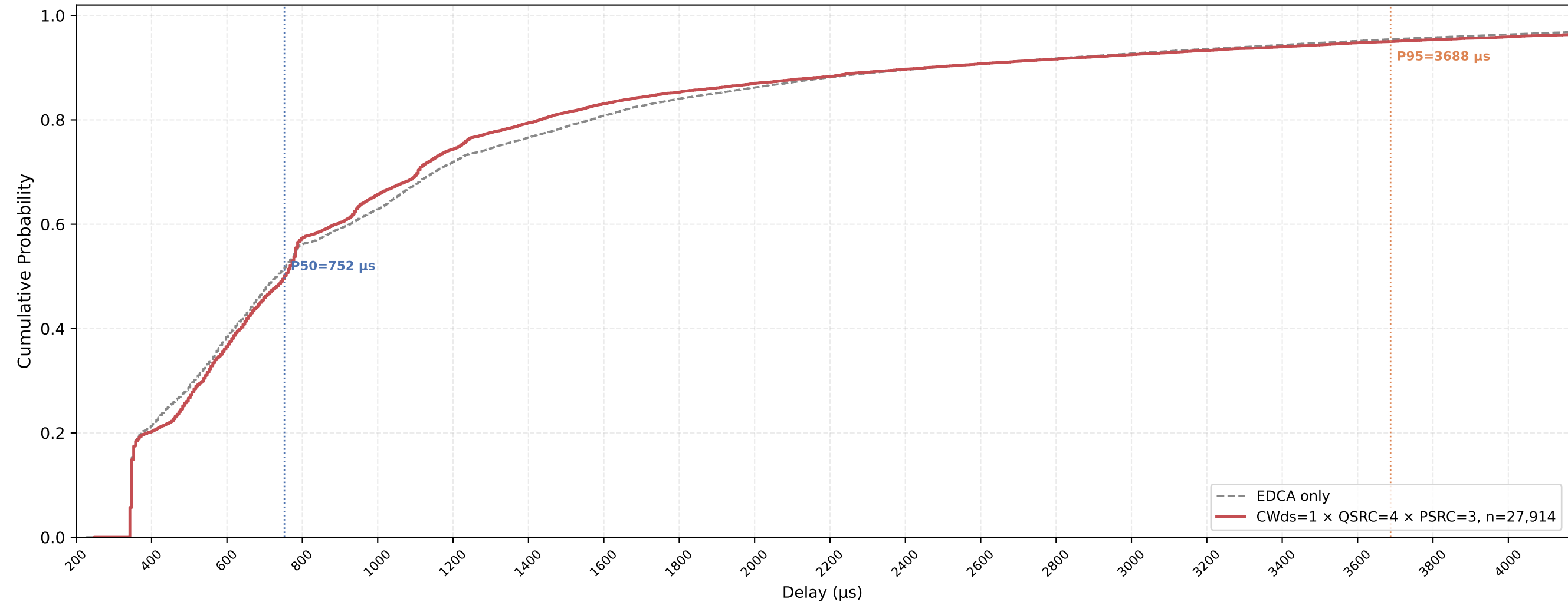
P-EDCA STA VO Delay CDF — CWds=1 × QSRC=4 × PSRC=3 nSta=30, nPedca=5, 0.5Mbps, avg of 10 runs
