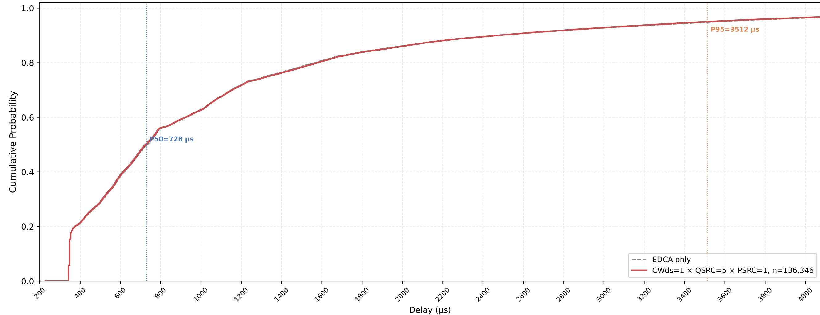
Legacy STA VO Delay CDF — CWds=1 × QSRC=5 × PSRC=1 nSta=30, nPedca=5, 0.5Mbps, avg of 10 runs
