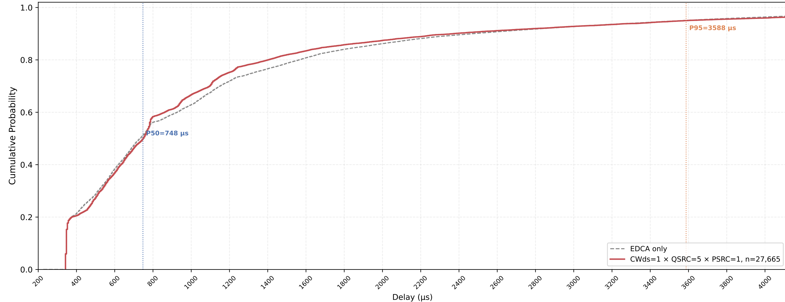
P-EDCA STA VO Delay CDF — CWds=1 × QSRC=5 × PSRC=1 nSta=30, nPedca=5, 0.5Mbps, avg of 10 runs
