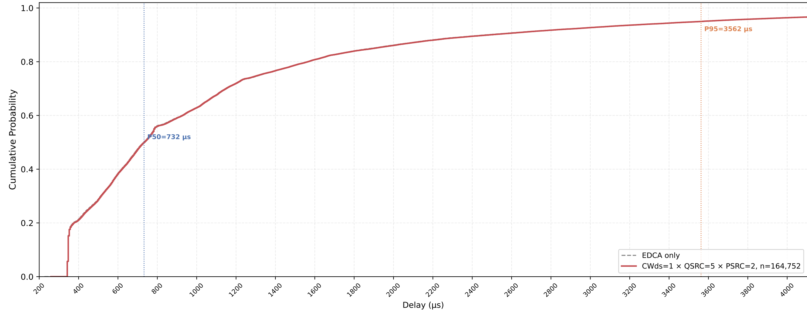
VO (all STAs) Delay CDF — CWds=1 × QSRC=5 × PSRC=2 nSta=30, nPedca=5, 0.5Mbps, avg of 10 runs
