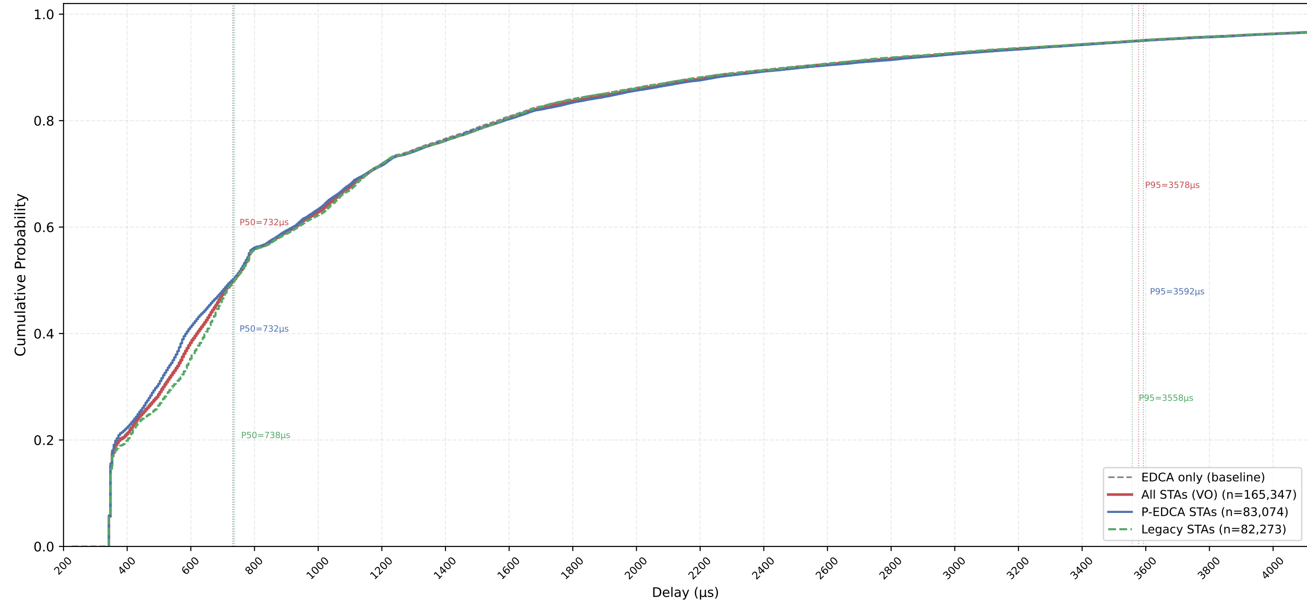
VO Delay CDF — P-EDCA / Legacy / All | CWds=1 × QSRC=5 × PSRC=3 nSta=30, nPedca=15/30, 0.5Mbps, avg of 10 runs
