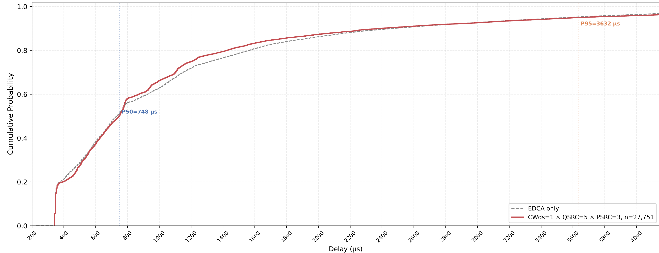
P-EDCA STA VO Delay CDF — CWds=1 × QSRC=5 × PSRC=3 nSta=30, nPedca=5, 0.5Mbps, avg of 10 runs
