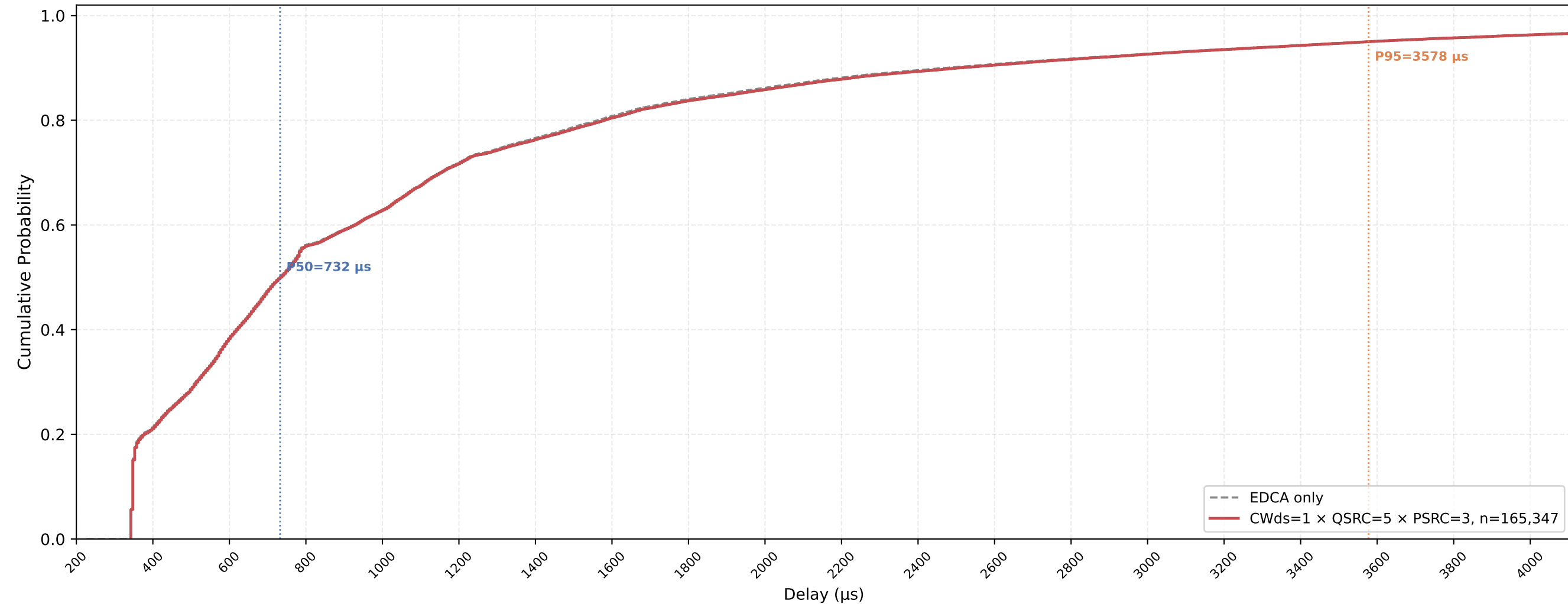
VO (all STAs) Delay CDF — CWds=1 × QSRC=5 × PSRC=3 nSta=30, nPedca=15, 0.5Mbps, avg of 10 runs
