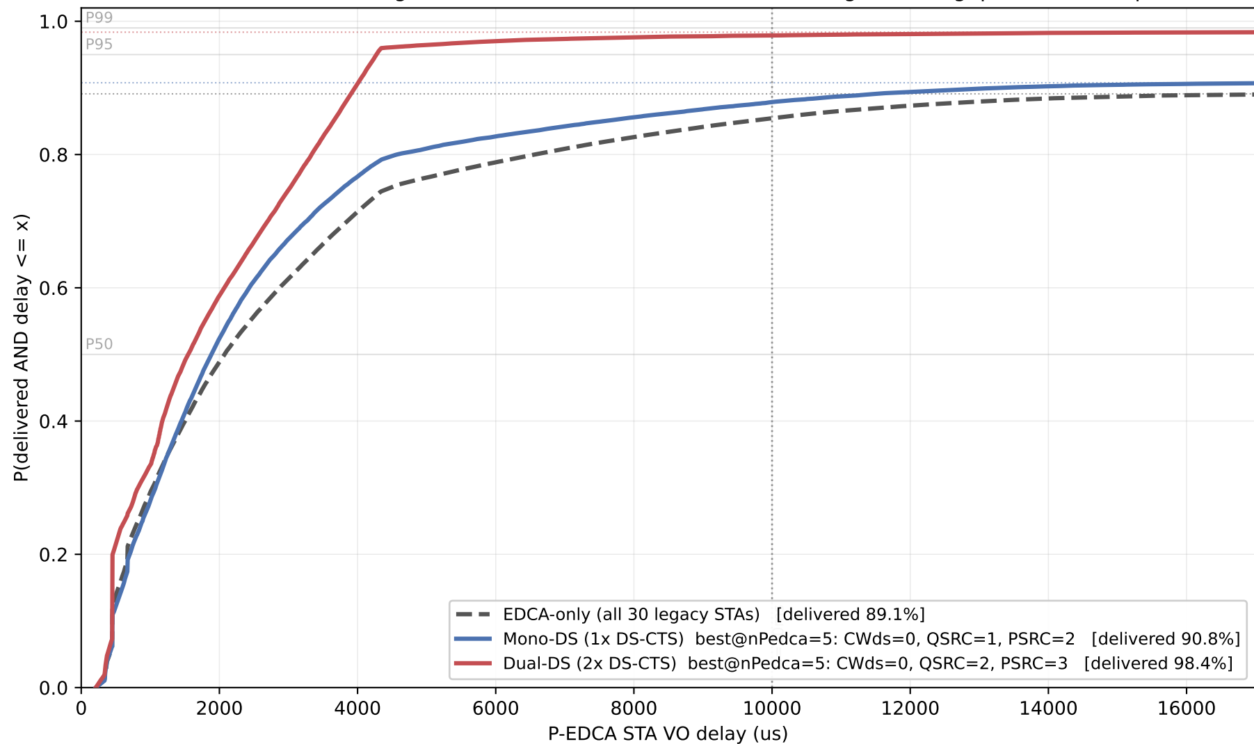
P-EDCA STA Delay CDF at Best Parameters (nPedca=5/30, nSta=30, 1Mbps) curves saturate at each configuration's delivered fraction (dotted ceilings) — the gap below 1.0 is packet loss
