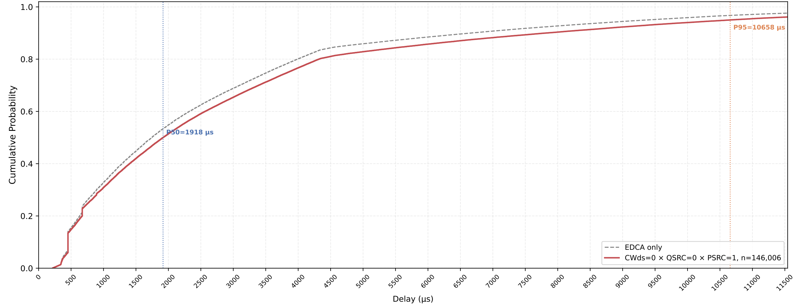
Legacy STA VO Delay CDF — CWds=0 × QSRC=0 × PSRC=1 nSta=30, nPedca=5, 1Mbps, avg of 10 runs
