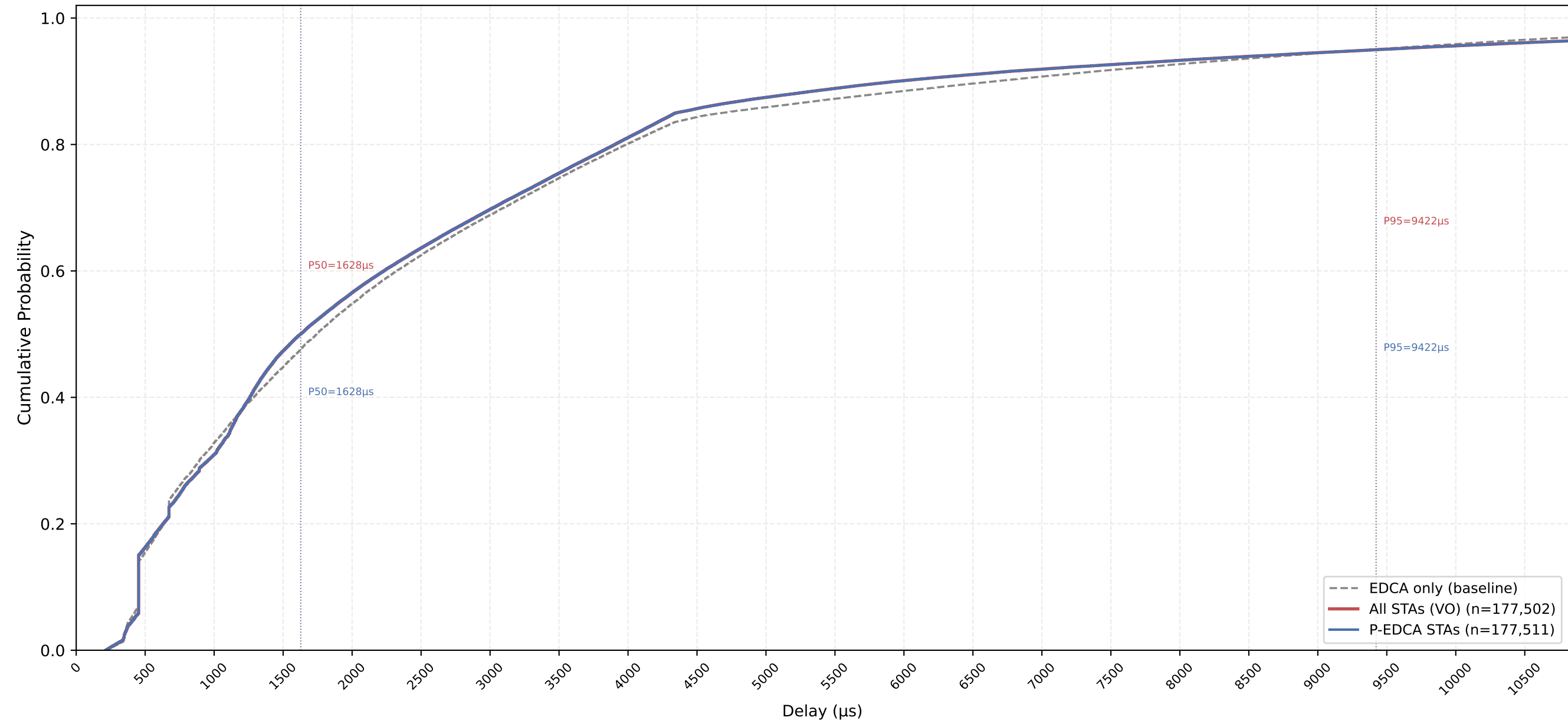
VO Delay CDF — P-EDCA / Legacy / All | CWds=0 × QSRC=3 × PSRC=1 nSta=30, nPedca=30/30, 1Mbps, avg of 10 runs
