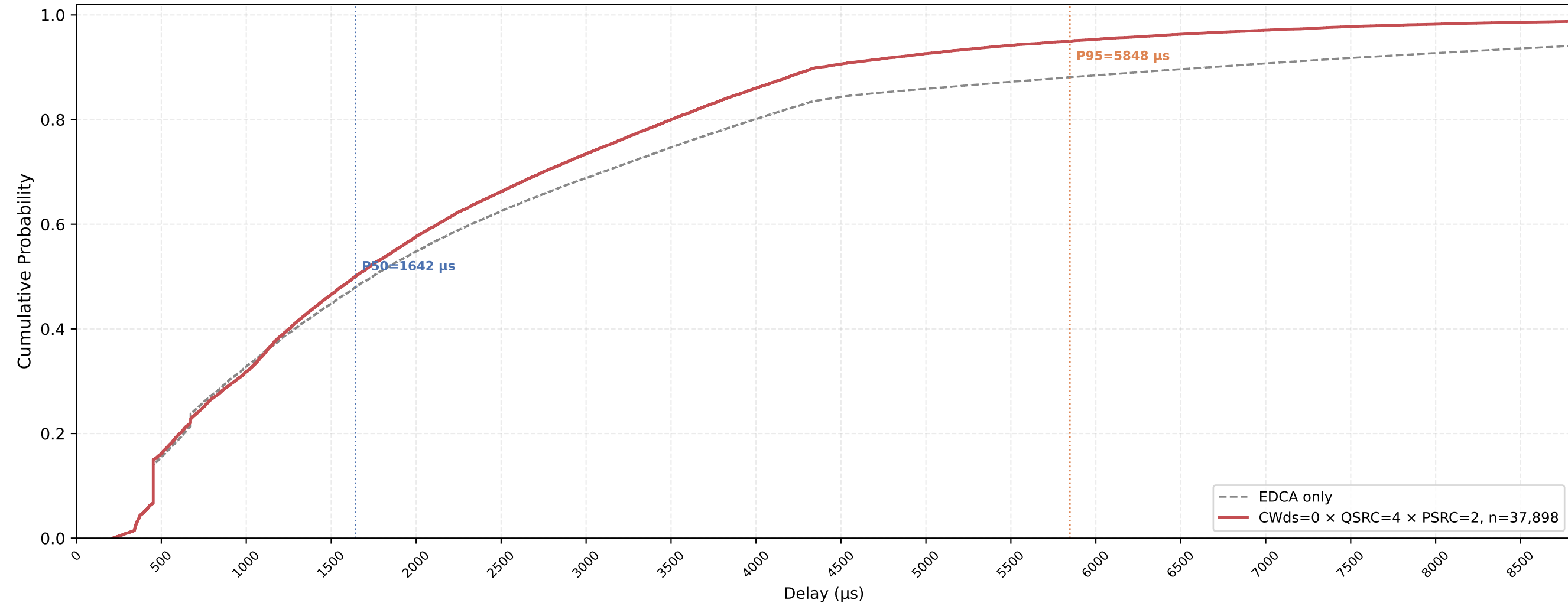
P-EDCA STA VO Delay CDF — CWds=0 × QSRC=4 × PSRC=2 nSta=30, nPedca=5, 1Mbps, avg of 10 runs
