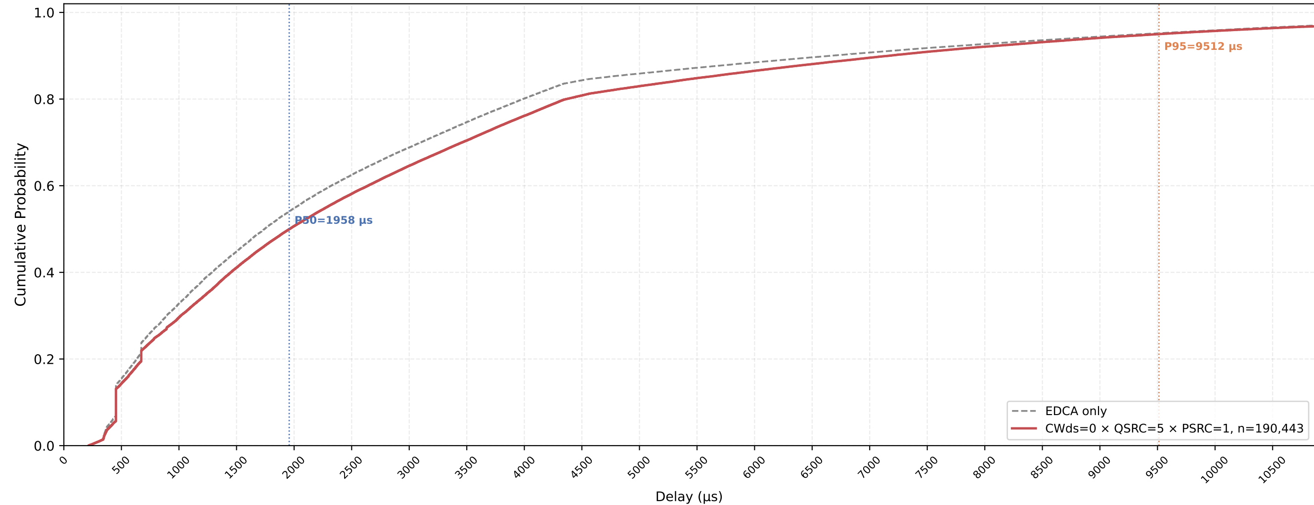
VO (all STAs) Delay CDF — CWds=0 × QSRC=5 × PSRC=1 nSta=30, nPedca=30, 1Mbps, avg of 10 runs
