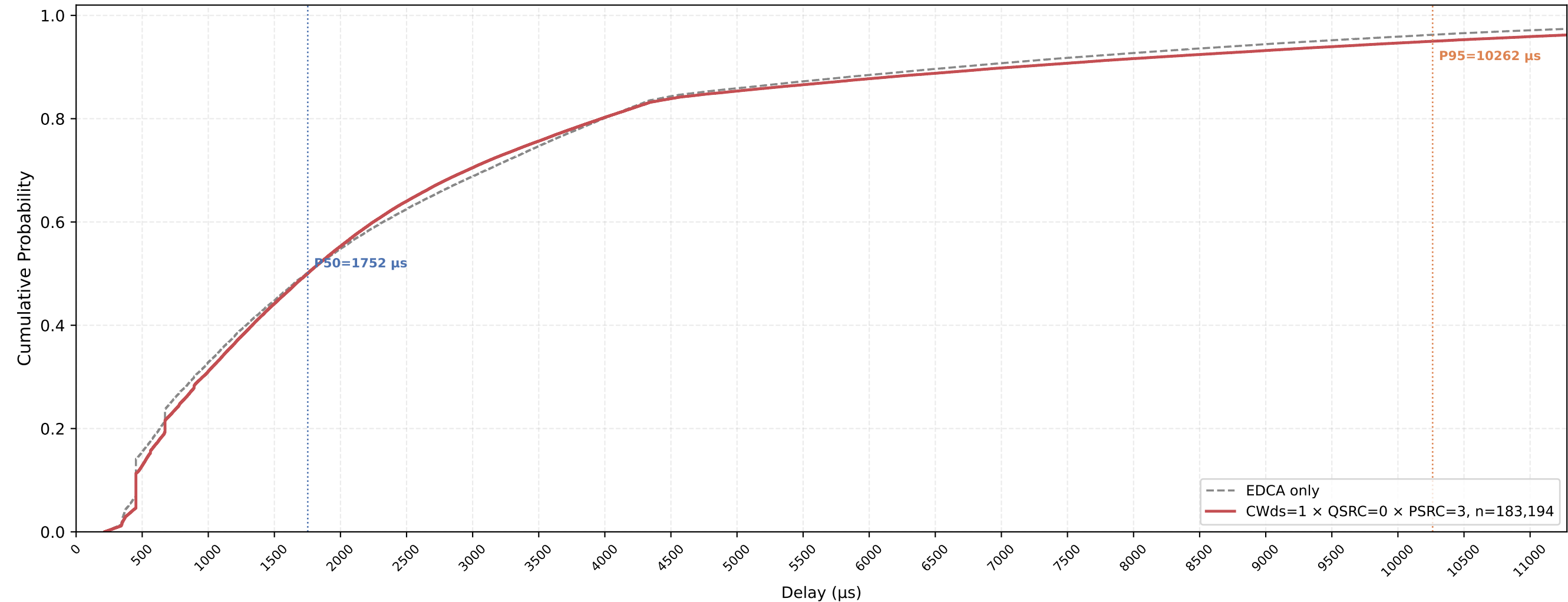
VO (all STAs) Delay CDF — CWds=1 × QSRC=0 × PSRC=3 nSta=30, nPedca=5, 1Mbps, avg of 10 runs
