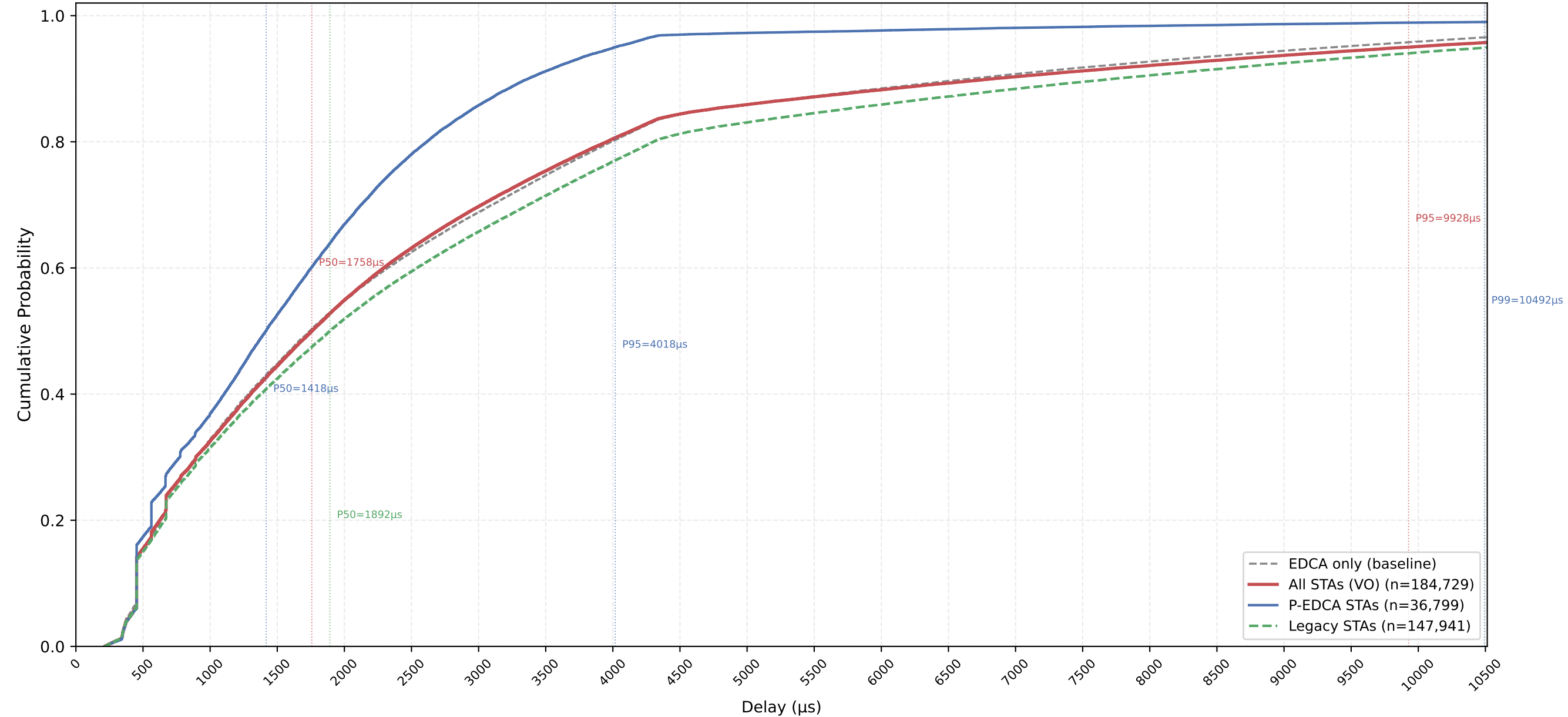
VO Delay CDF — P-EDCA / Legacy / All | CWds=1 × QSRC=1 × PSRC=3 nSta=30, nPedca=5/30, 1Mbps, avg of 10 runs
