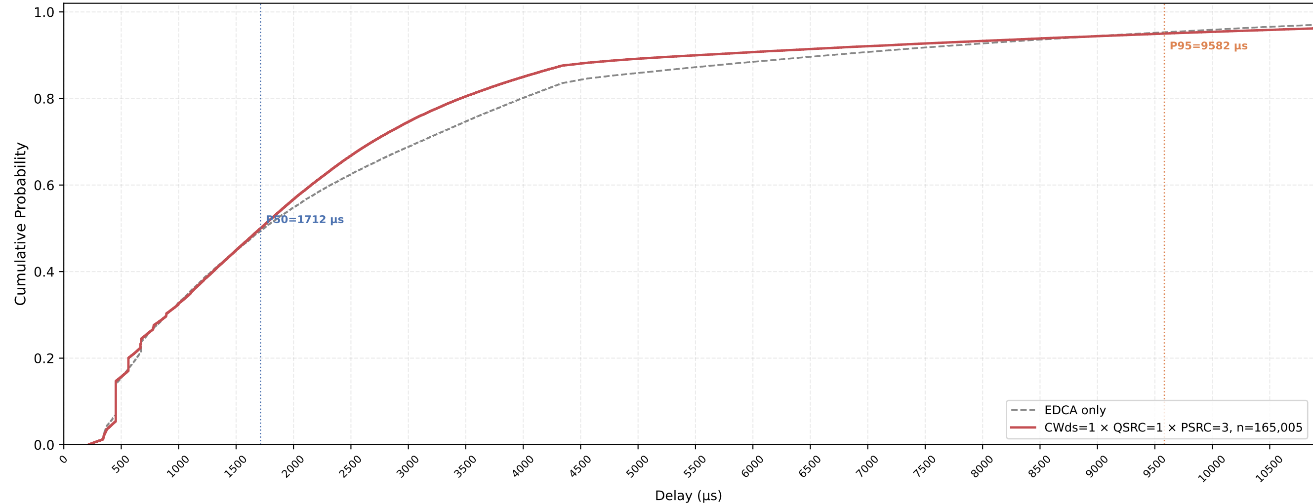
P-EDCA STA VO Delay CDF — CWds=1 × QSRC=1 × PSRC=3 nSta=30, nPedca=30, 1Mbps, avg of 10 runs
