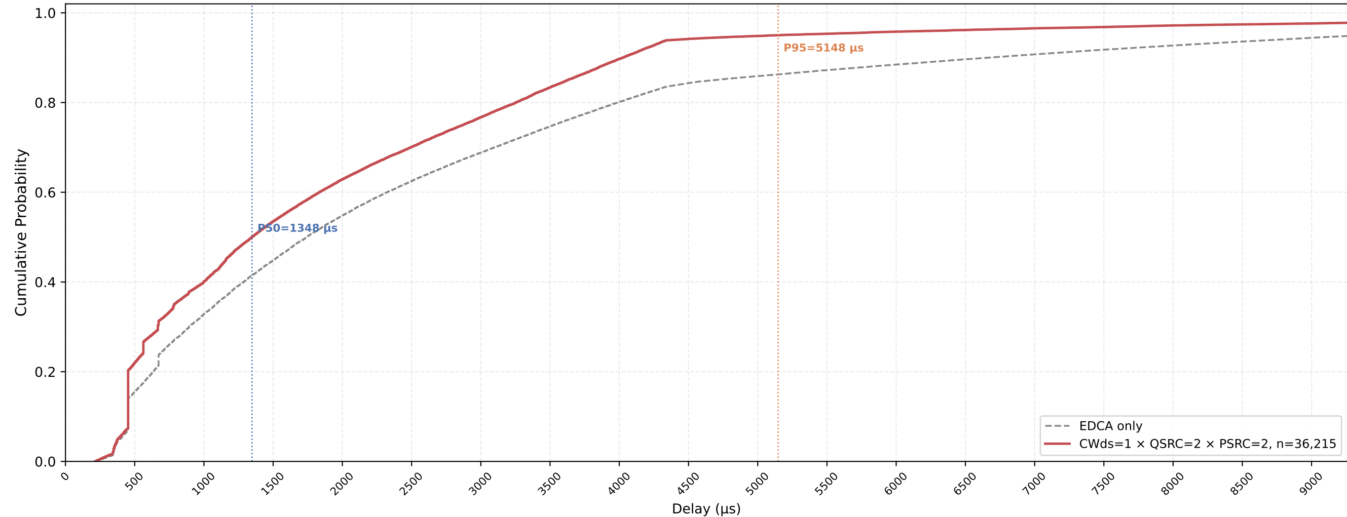
P-EDCA STA VO Delay CDF — CWds=1 × QSRC=2 × PSRC=2 nSta=30, nPedca=5, 1Mbps, avg of 10 runs
