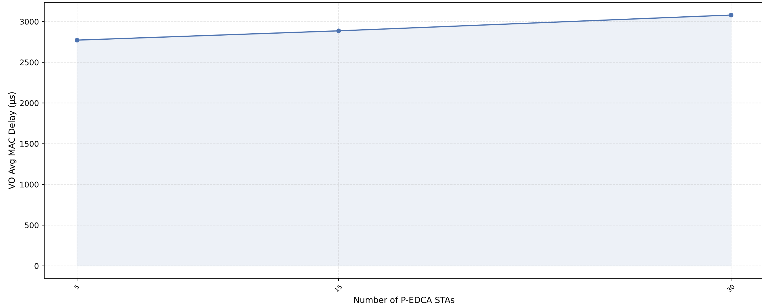
VO Avg MAC Delay vs P-EDCA STAs — nSta=30, 1Mbps (avg of 10 runs)
