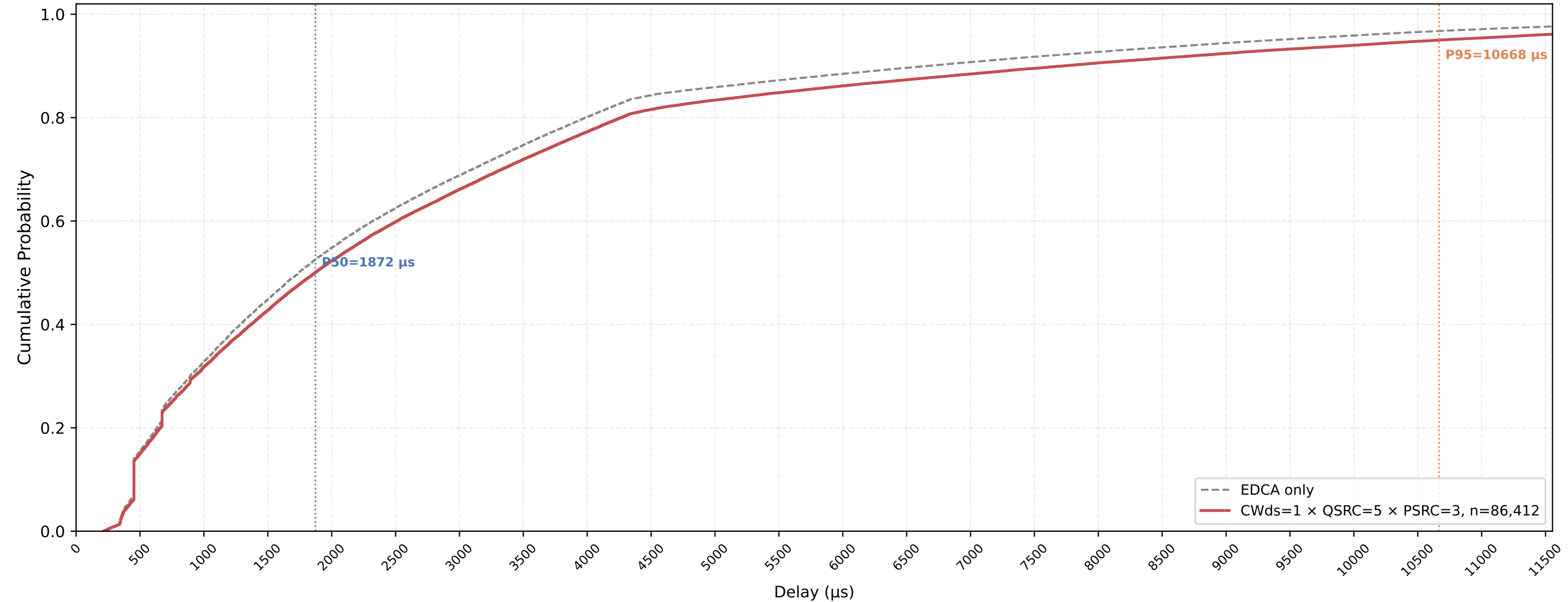
Legacy STA VO Delay CDF — CWds=1 × QSRC=5 × PSRC=3 nSta=30, nPedca=15, 1Mbps, avg of 10 runs
