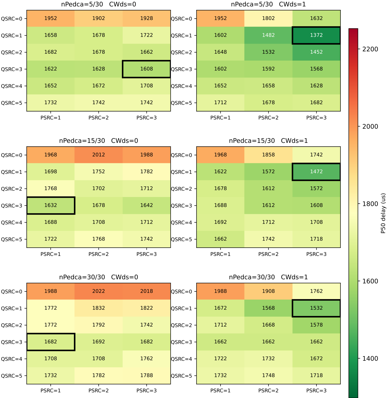
P-EDCA STA VO Delay — Median Mono-DS (1x DS-CTS) (nSta=30, 1Mbps, black box = best in panel) colour scale 1298-2252 shared across mono-DS & dual-DS — panels are directly comparable
