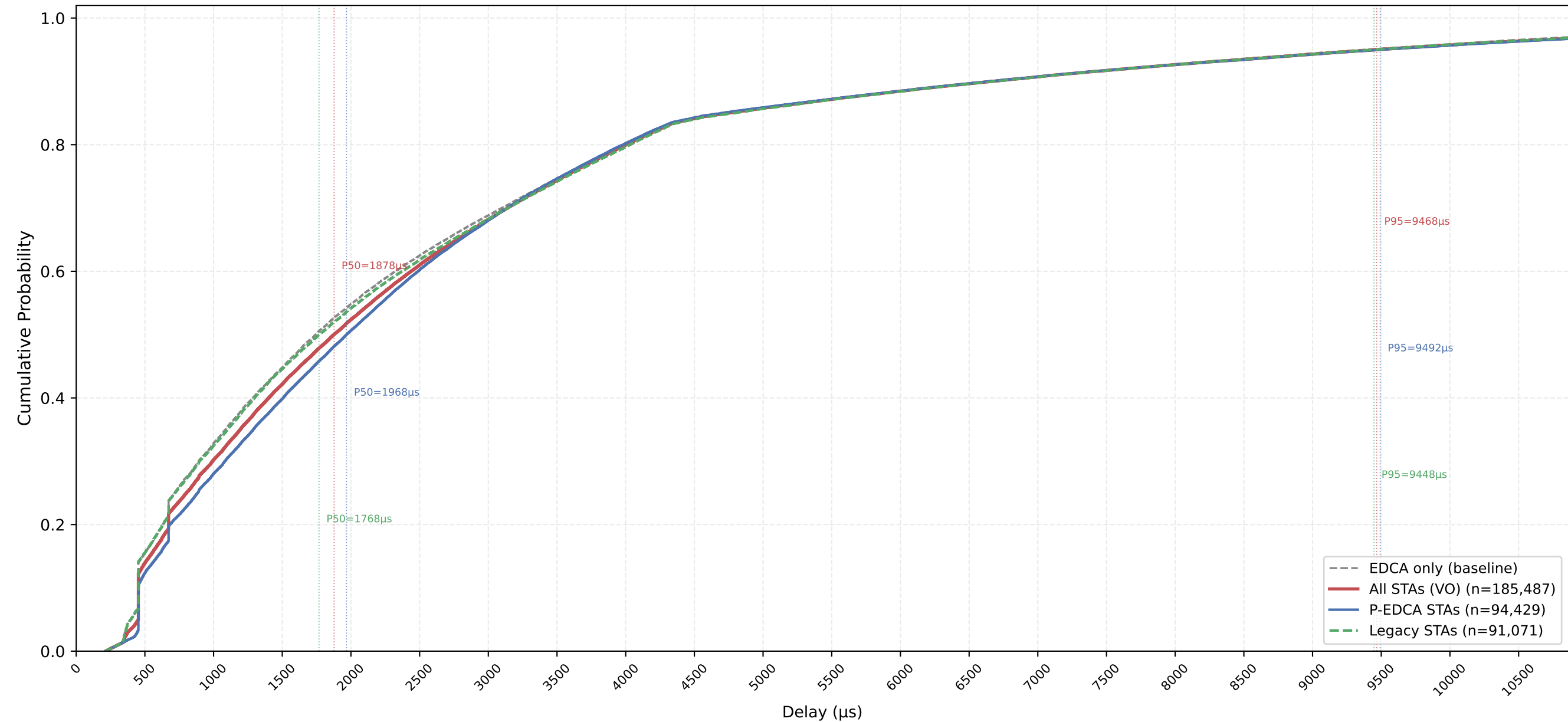
VO Delay CDF — P-EDCA / Legacy / All | CWds=0 × QSRC=0 × PSRC=1 nSta=30, nPedca=15/30, 1Mbps, avg of 10 runs
