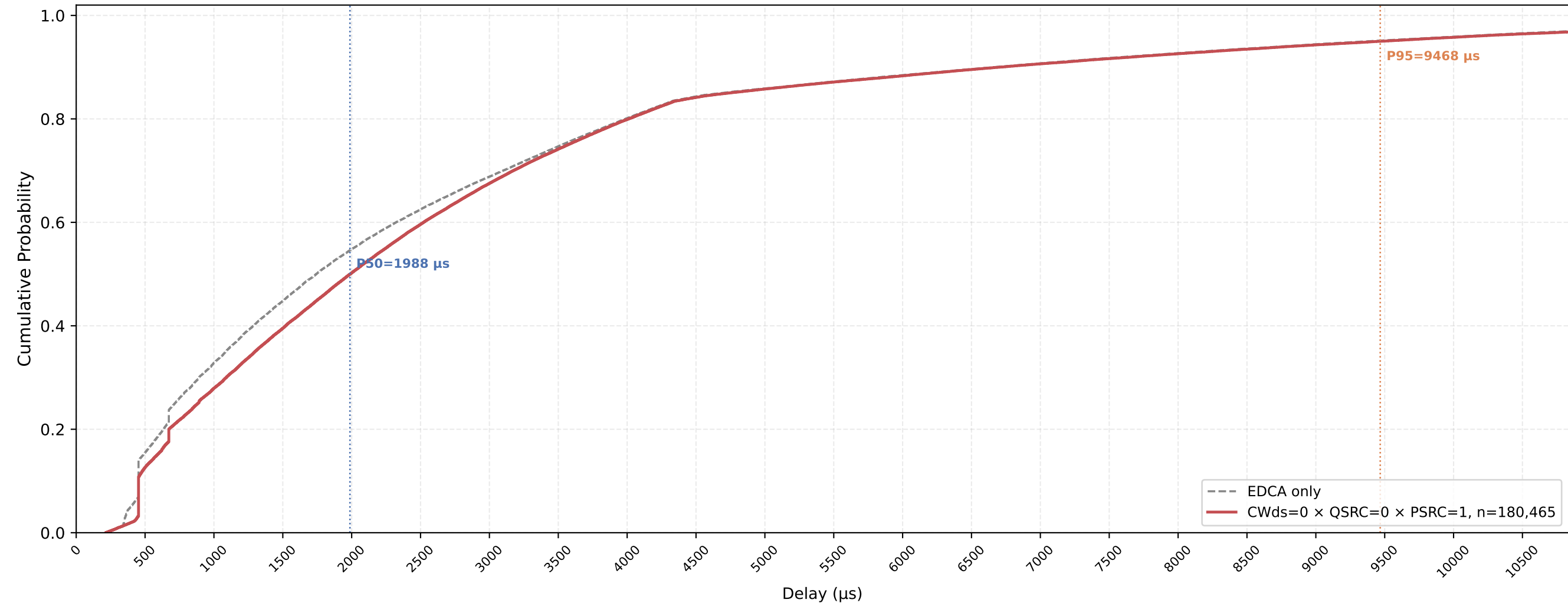
VO (all STAs) Delay CDF — CWds=0 × QSRC=0 × PSRC=1 nSta=30, nPedca=30, 1Mbps, avg of 10 runs
