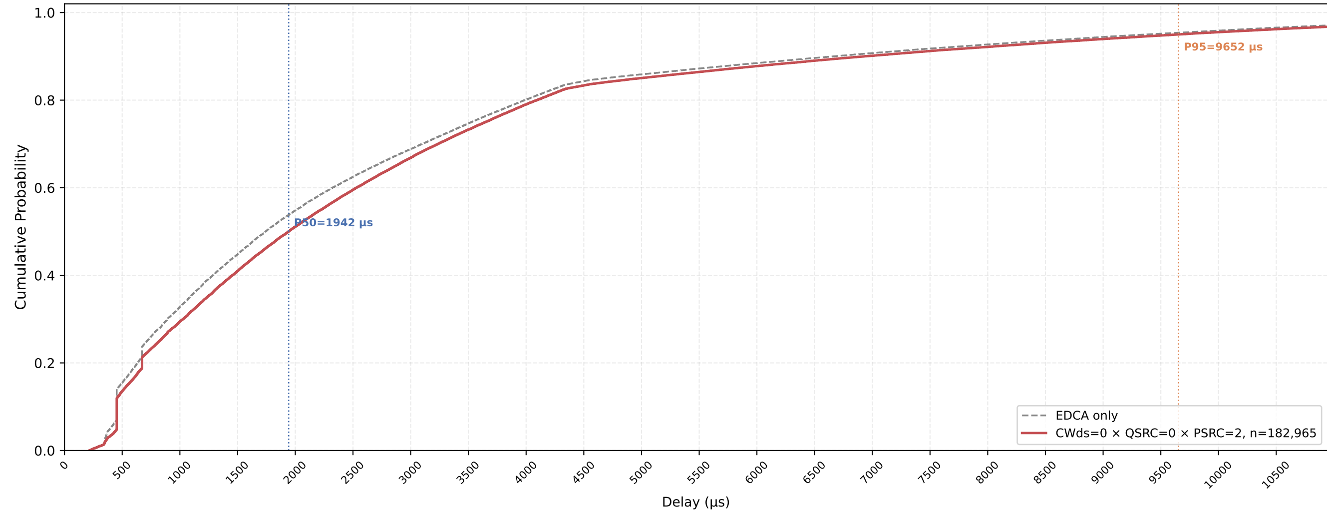
VO (all STAs) Delay CDF — CWds=0 × QSRC=0 × PSRC=2 nSta=30, nPedca=15, 1Mbps, avg of 10 runs
