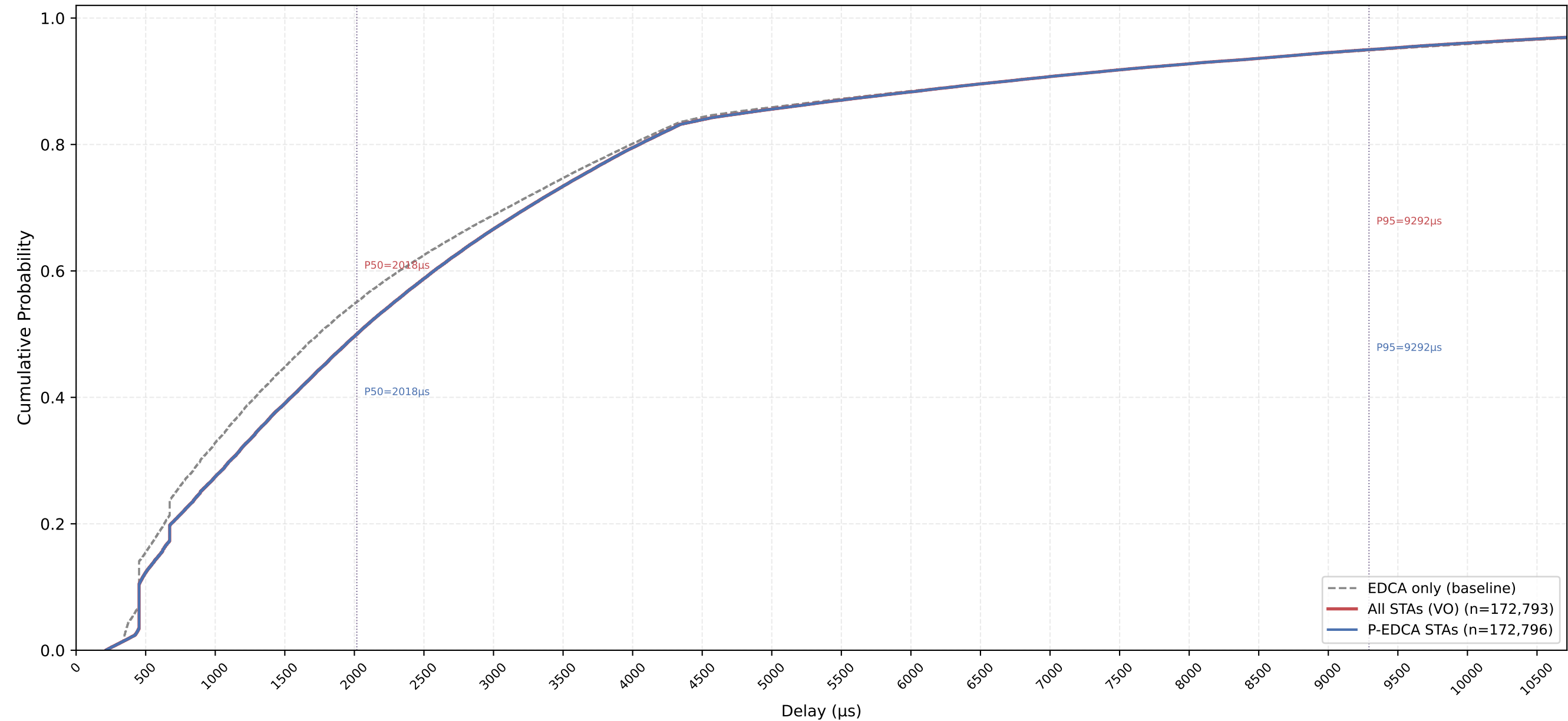
VO Delay CDF — P-EDCA / Legacy / All | CWds=0 × QSRC=0 × PSRC=3 nSta=30, nPedca=30/30, 1Mbps, avg of 10 runs
