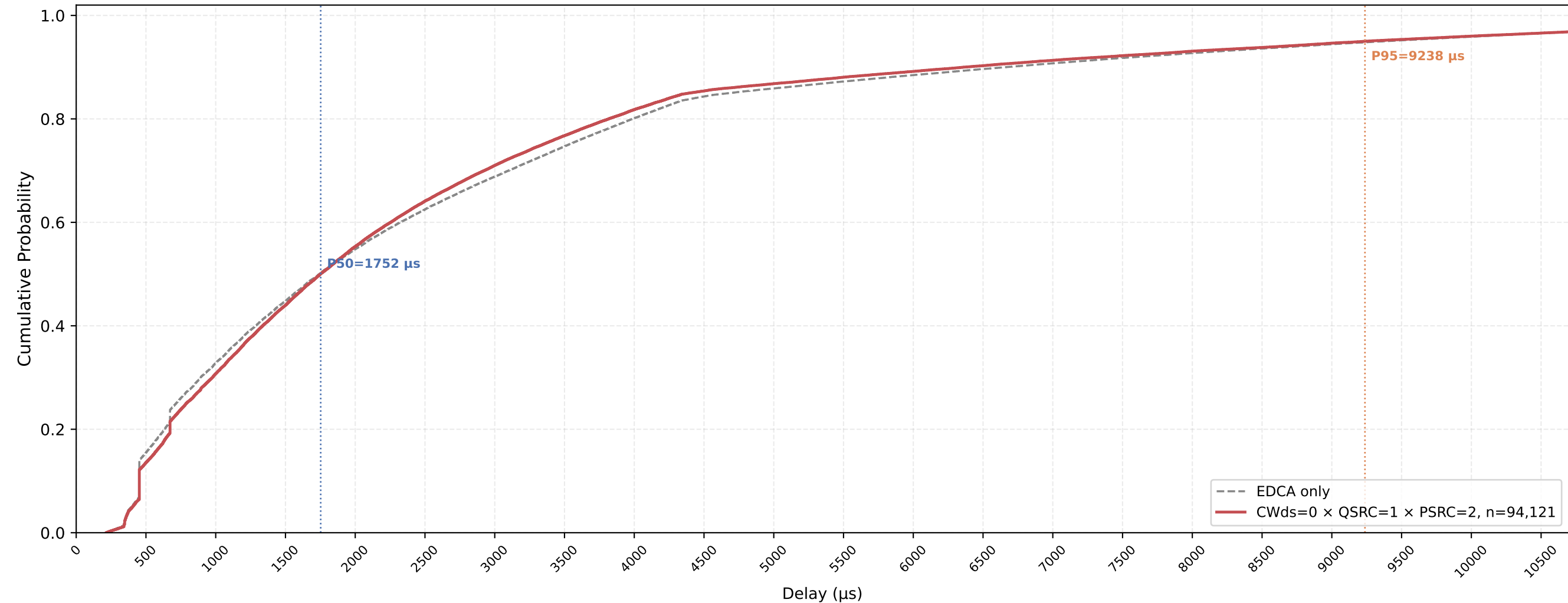
P-EDCA STA VO Delay CDF — CWds=0 × QSRC=1 × PSRC=2 nSta=30, nPedca=15, 1Mbps, avg of 10 runs
