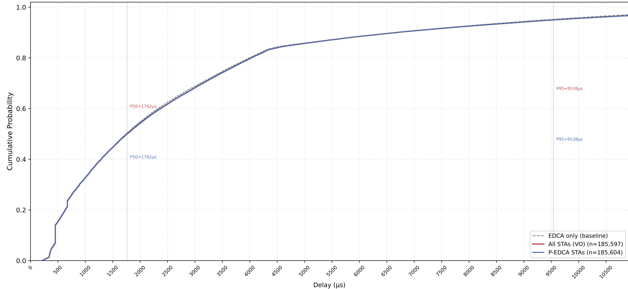
VO Delay CDF — P-EDCA / Legacy / All | CWds=0 × QSRC=4 × PSRC=3 nSta=30, nPedca=30/30, 1Mbps, avg of 10 runs
