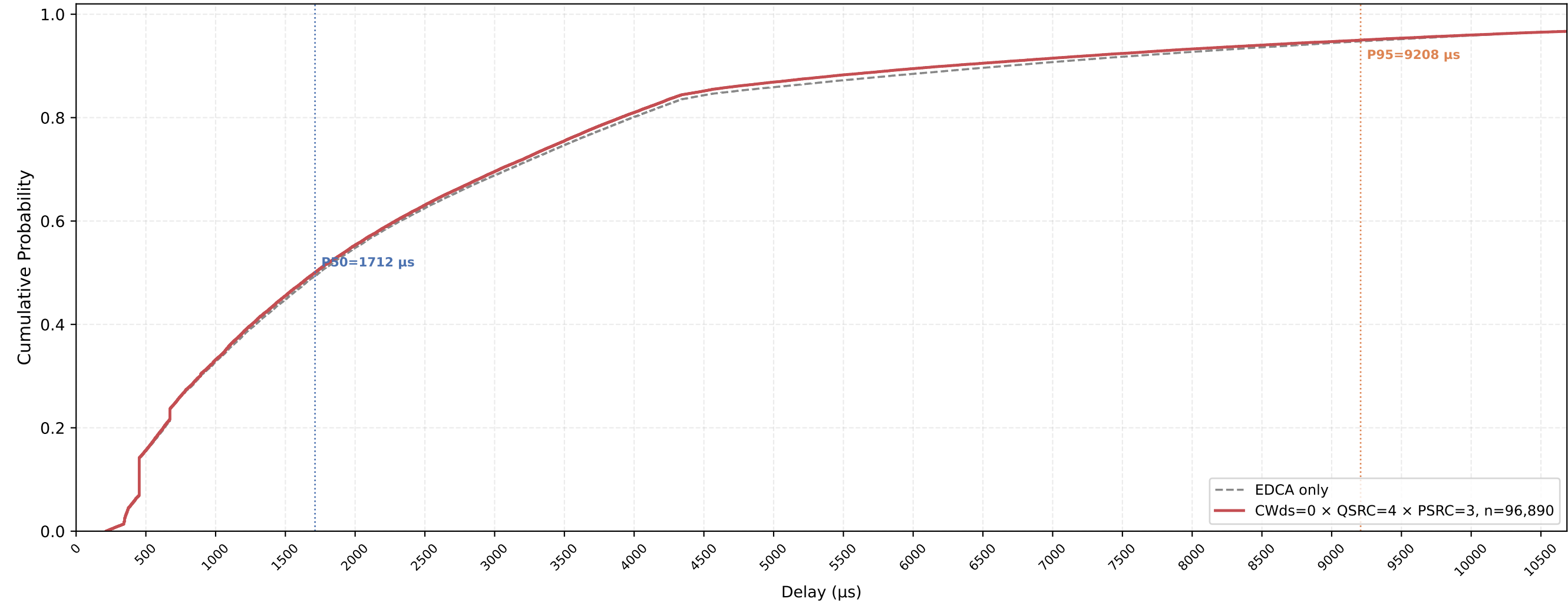
P-EDCA STA VO Delay CDF — CWds=0 × QSRC=4 × PSRC=3 nSta=30, nPedca=15, 1Mbps, avg of 10 runs
