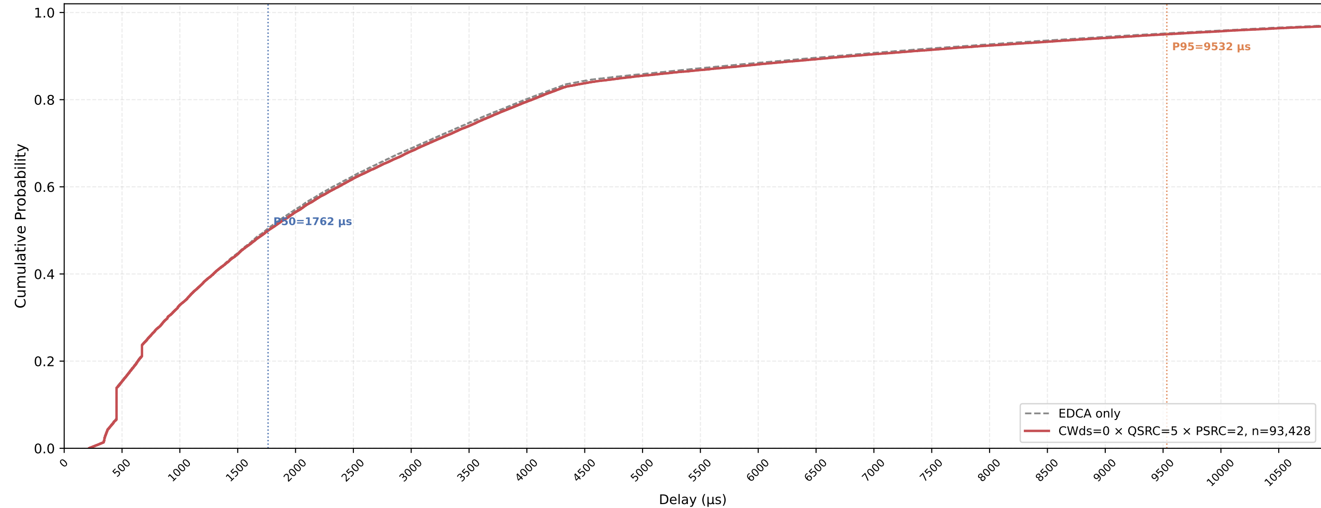
Legacy STA VO Delay CDF — CWds=0 × QSRC=5 × PSRC=2 nSta=30, nPedca=15, 1Mbps, avg of 10 runs
