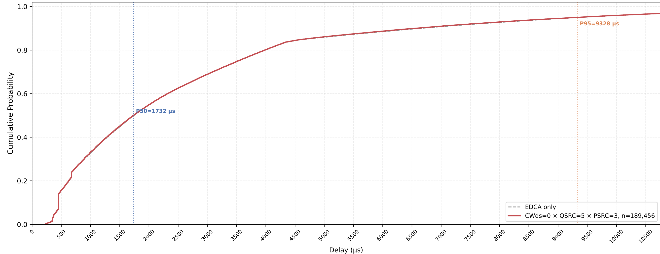
VO (all STAs) Delay CDF — CWds=0 × QSRC=5 × PSRC=3 nSta=30, nPedca=15, 1Mbps, avg of 10 runs
