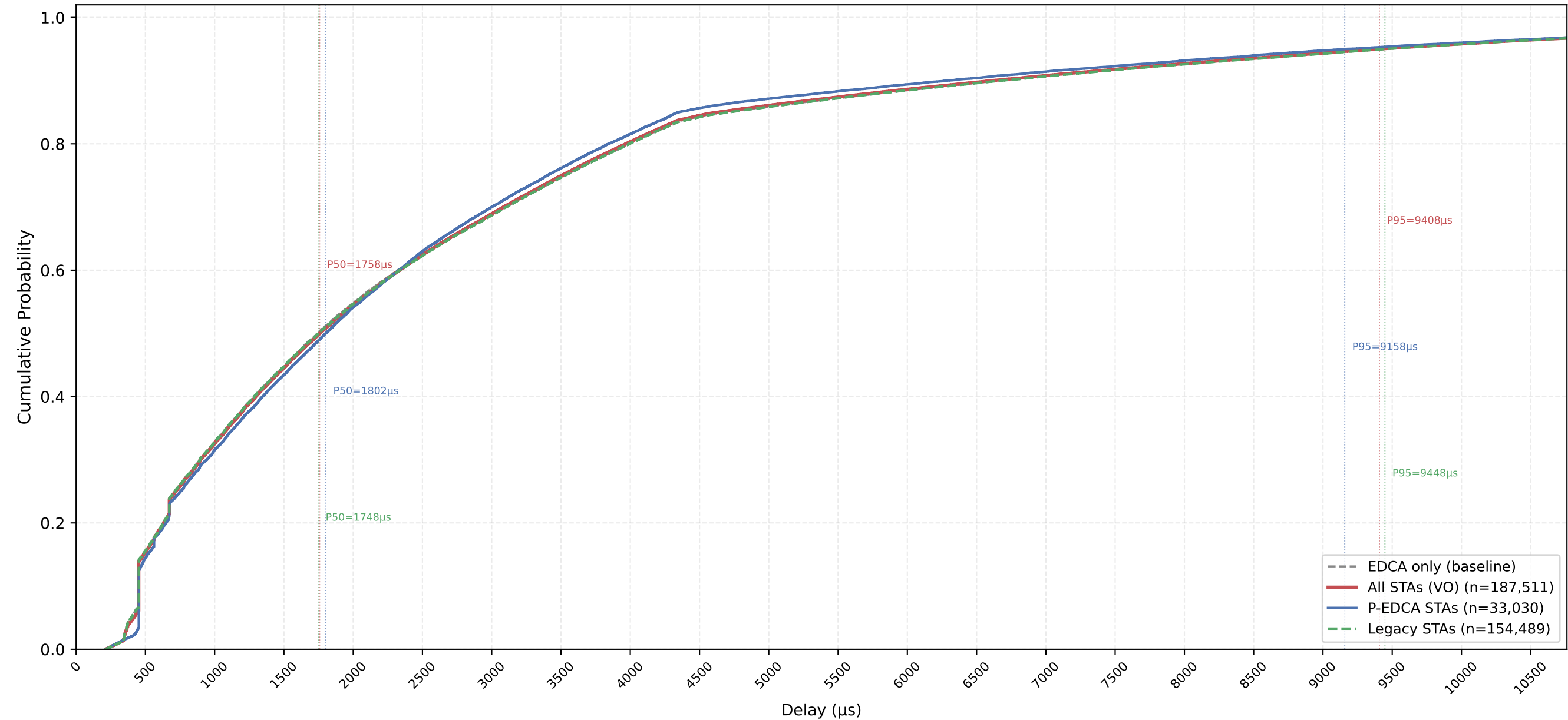
VO Delay CDF — P-EDCA / Legacy / All | CWds=1 × QSRC=0 × PSRC=2 nSta=30, nPedca=5/30, 1Mbps, avg of 10 runs
