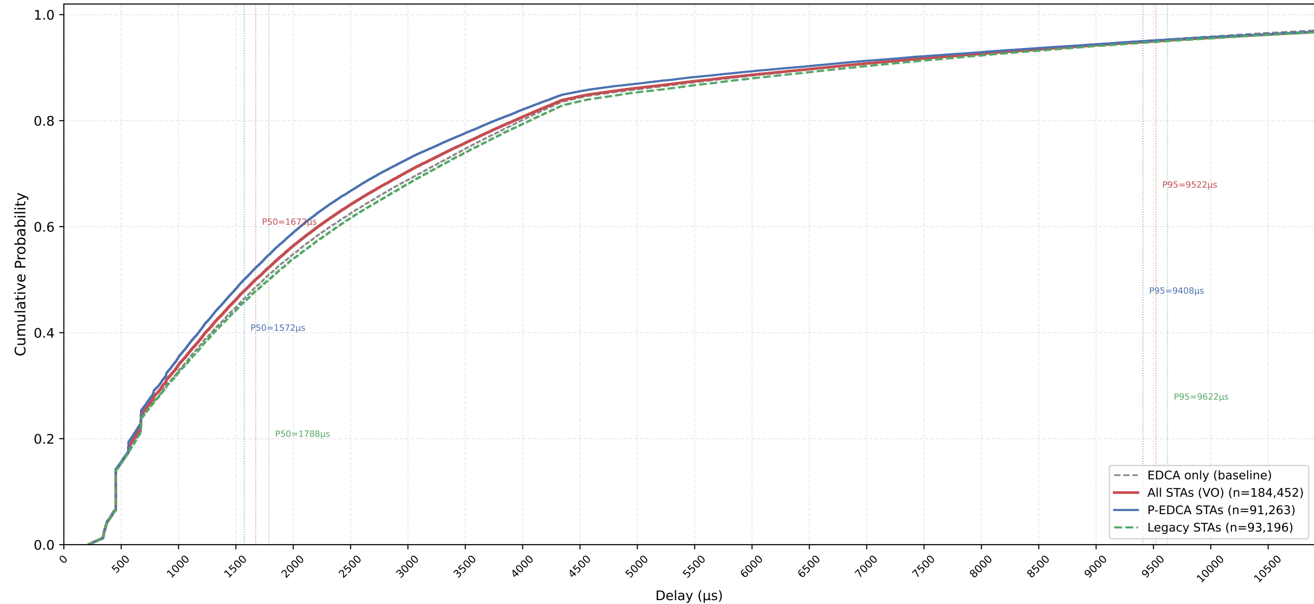
VO Delay CDF — P-EDCA / Legacy / All | CWds=1 × QSRC=1 × PSRC=2 nSta=30, nPedca=15/30, 1Mbps, avg of 10 runs
