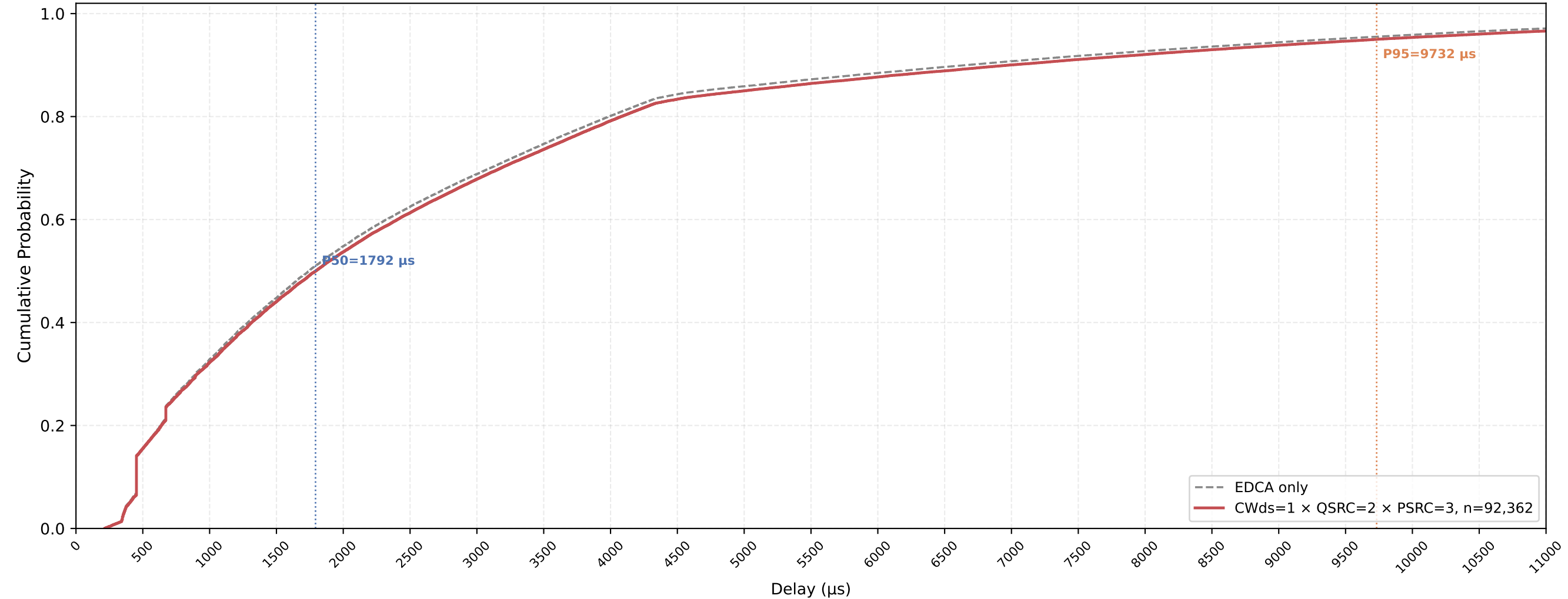
Legacy STA VO Delay CDF — CWds=1 × QSRC=2 × PSRC=3 nSta=30, nPedca=15, 1Mbps, avg of 10 runs
