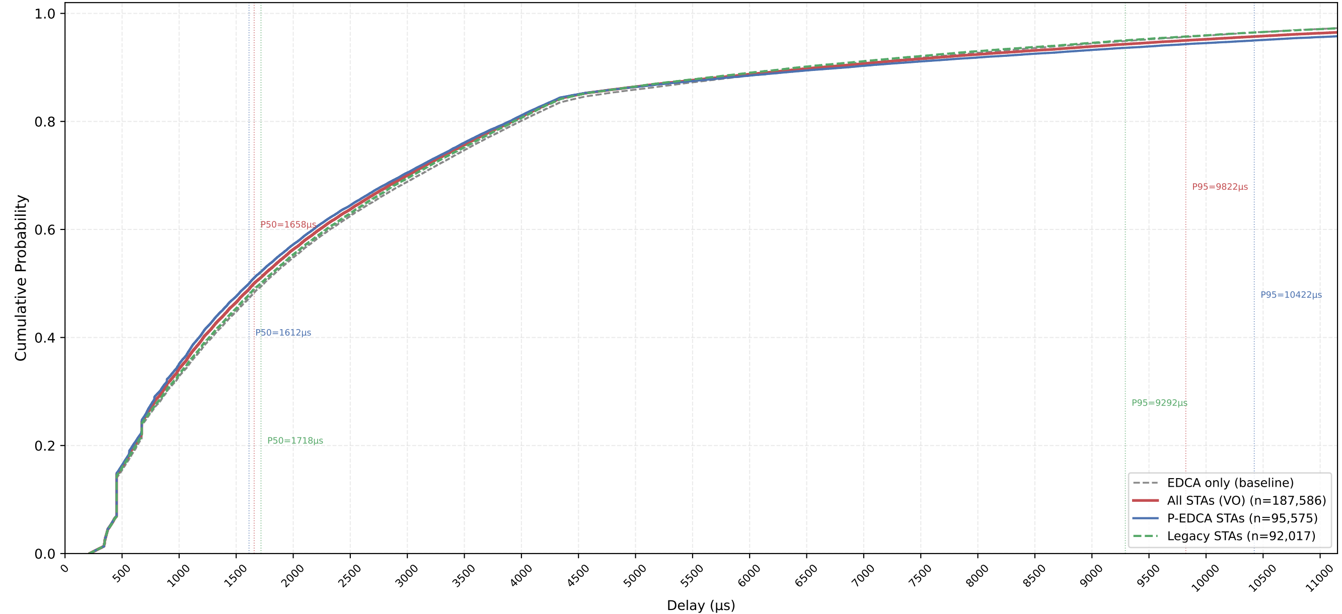
VO Delay CDF — P-EDCA / Legacy / All | CWds=1 × QSRC=3 × PSRC=2 nSta=30, nPedca=15/30, 1Mbps, avg of 10 runs
