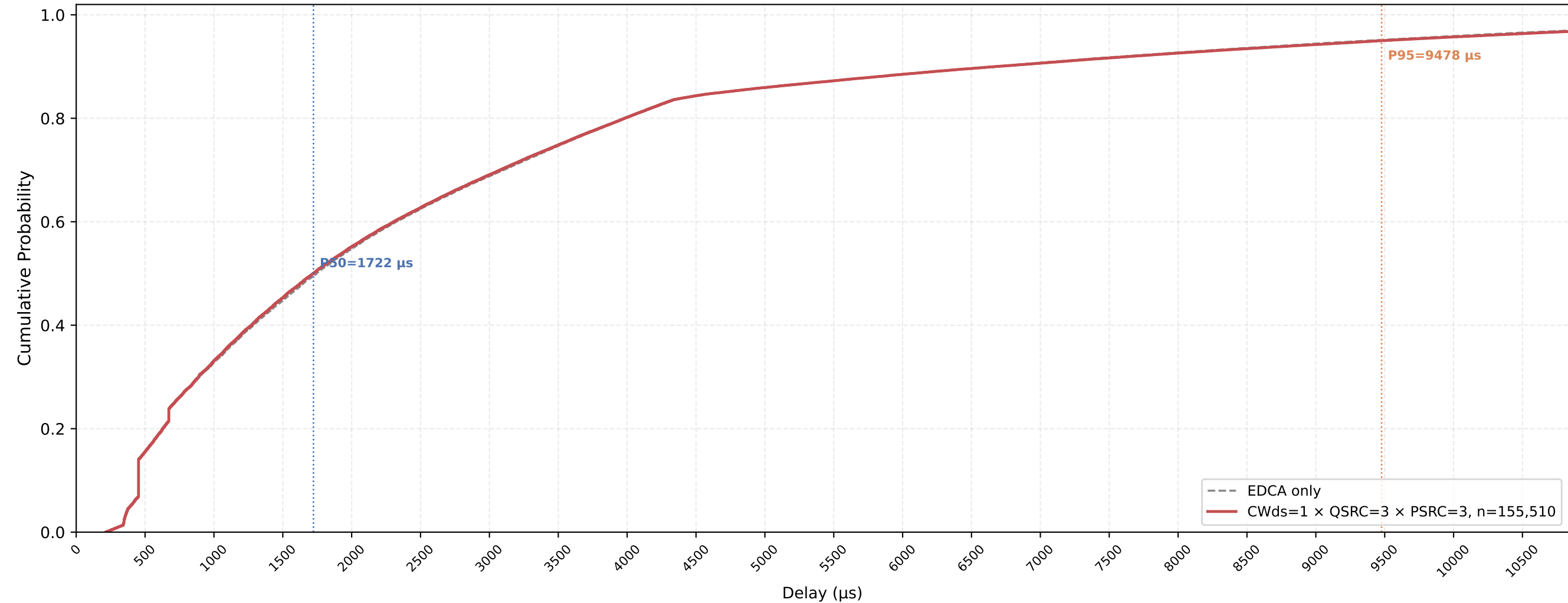
Legacy STA VO Delay CDF — CWds=1 × QSRC=3 × PSRC=3 nSta=30, nPedca=5, 1Mbps, avg of 10 runs
