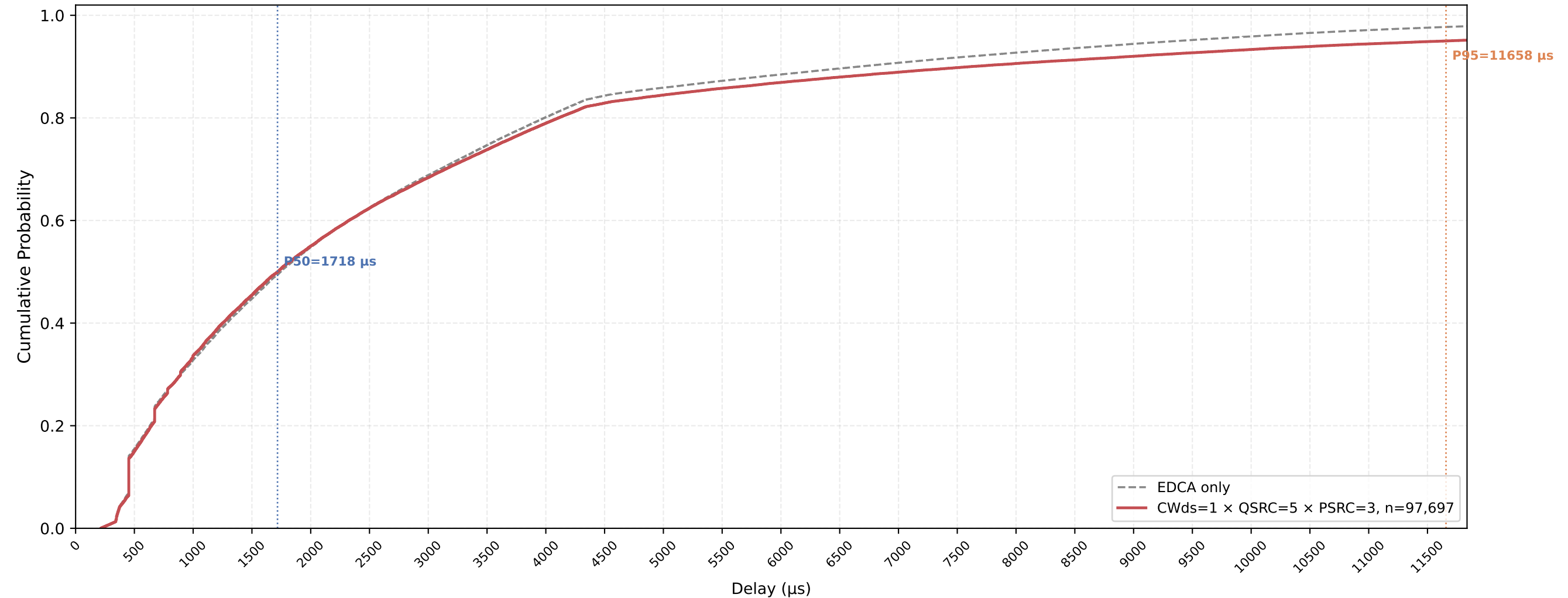
P-EDCA STA VO Delay CDF — CWds=1 × QSRC=5 × PSRC=3 nSta=30, nPedca=15, 1Mbps, avg of 10 runs
