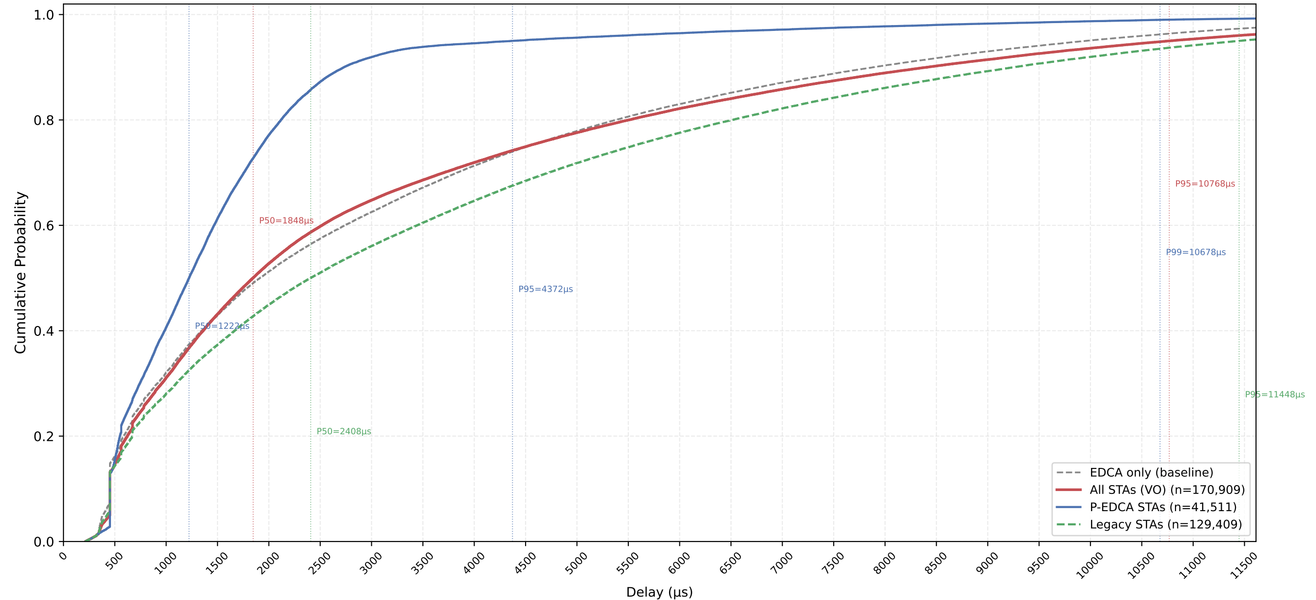
VO Delay CDF — P-EDCA / Legacy / All | CWds=0 × QSRC=0 × PSRC=2 nSta=30, nPedca=5/30, 1Mbps, avg of 10 runs
