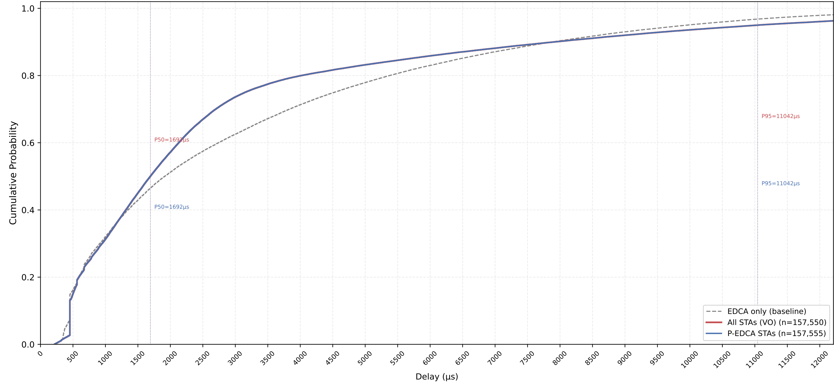
VO Delay CDF — P-EDCA / Legacy / All | CWds=0 × QSRC=0 × PSRC=2 nSta=30, nPedca=30/30, 1Mbps, avg of 10 runs
