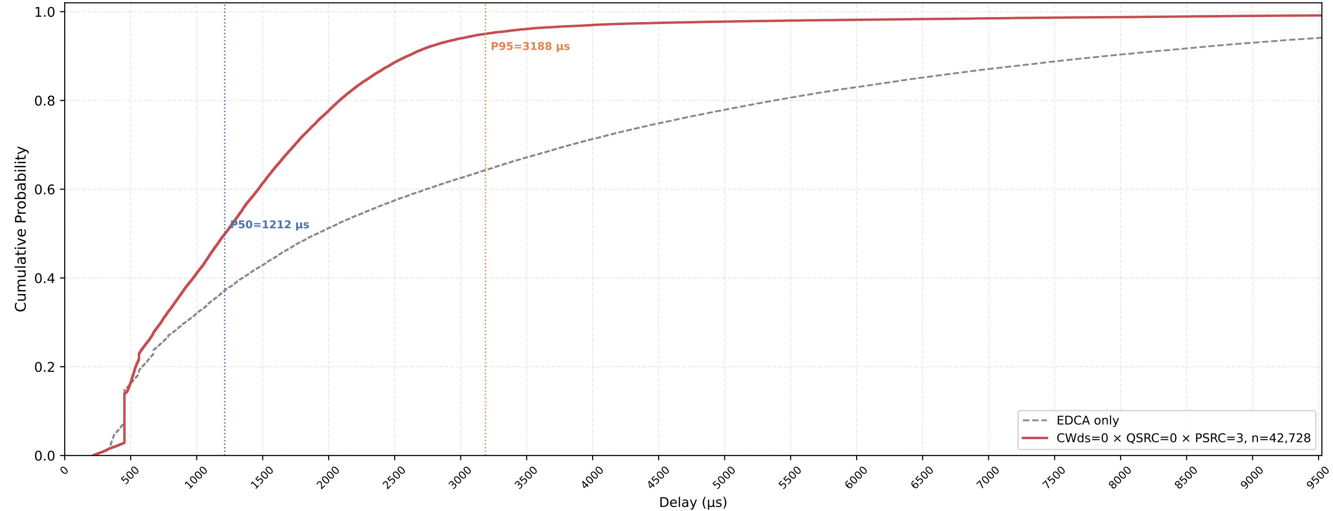
P-EDCA STA VO Delay CDF — CWds=0 × QSRC=0 × PSRC=3 nSta=30, nPedca=5, 1Mbps, avg of 10 runs
