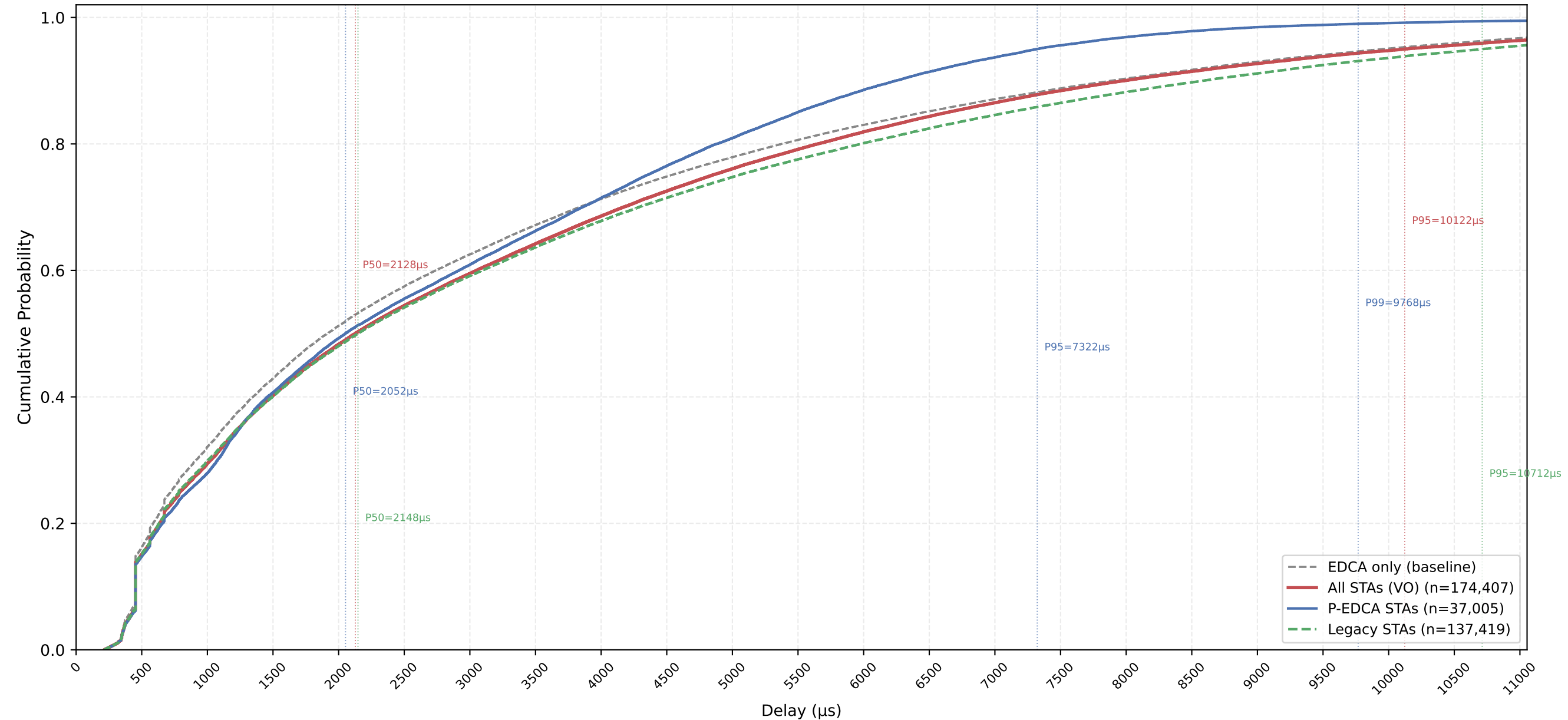
VO Delay CDF — P-EDCA / Legacy / All | CWds=0 × QSRC=3 × PSRC=2 nSta=30, nPedca=5/30, 1Mbps, avg of 10 runs
