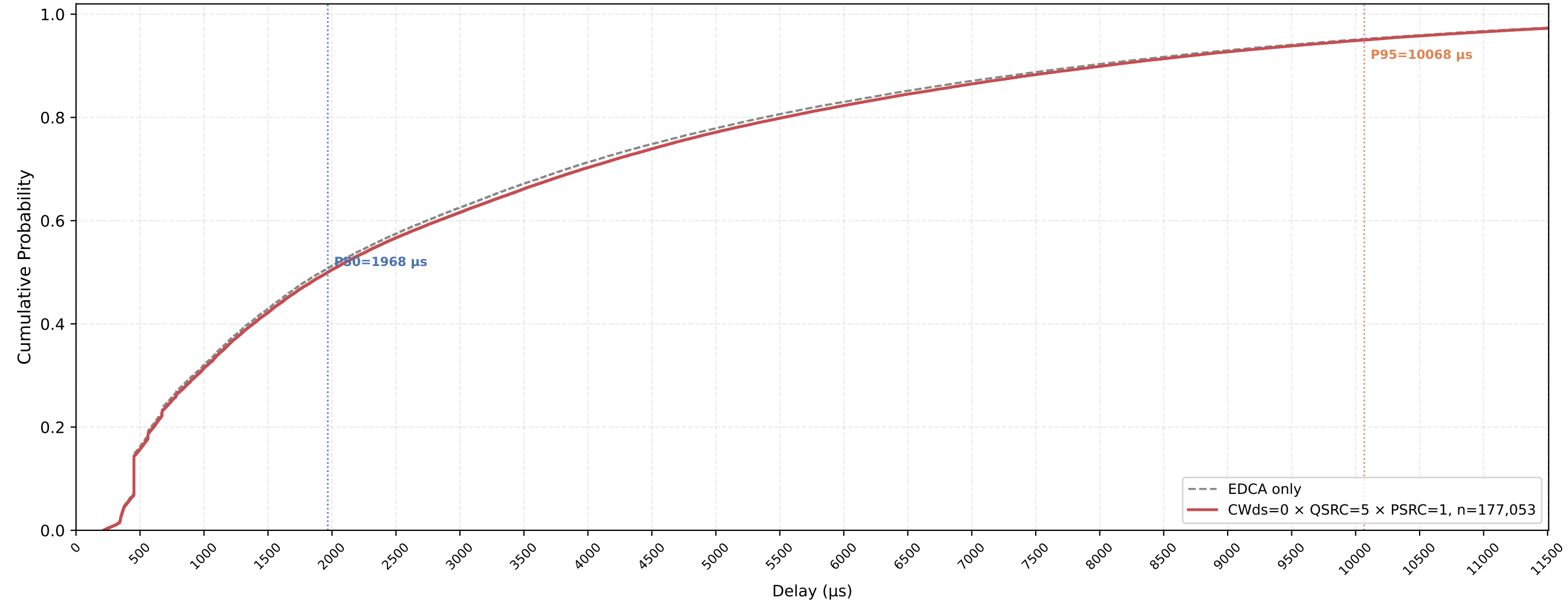
VO (all STAs) Delay CDF — CWds=0 × QSRC=5 × PSRC=1 nSta=30, nPedca=5, 1Mbps, avg of 10 runs
