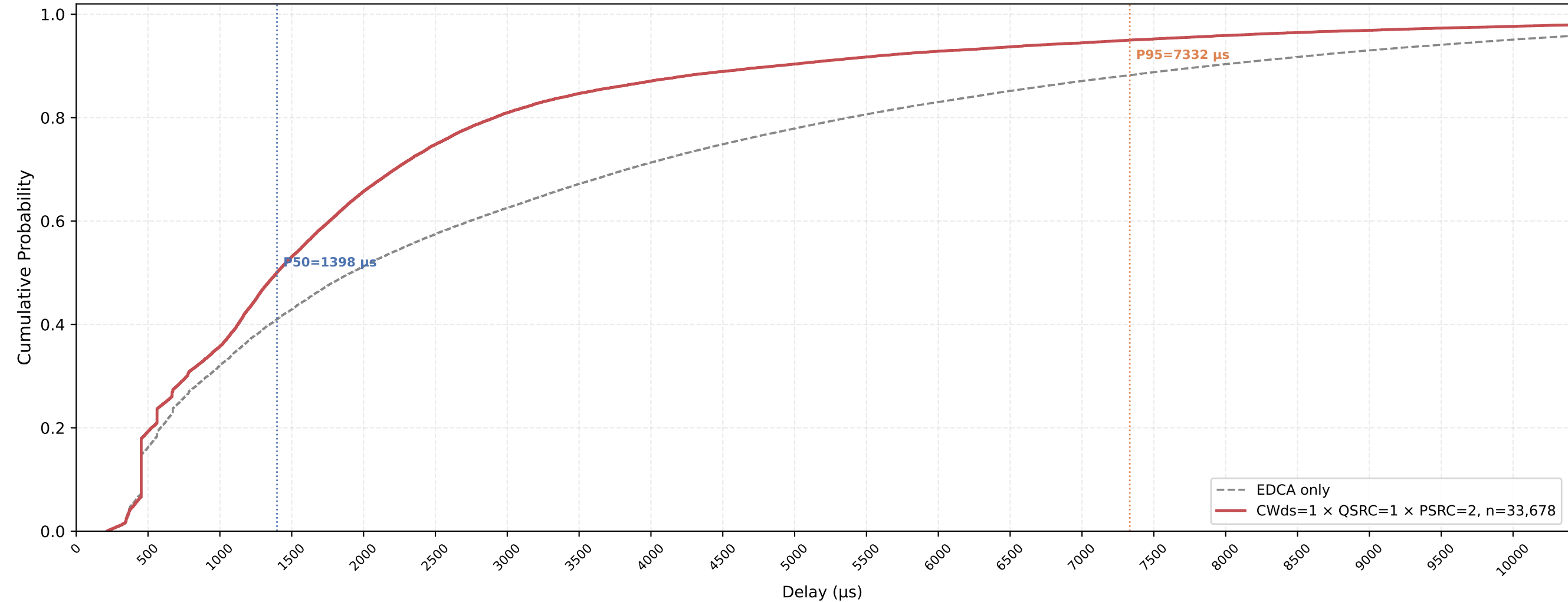
P-EDCA STA VO Delay CDF — CWds=1 × QSRC=1 × PSRC=2 nSta=30, nPedca=5, 1Mbps, avg of 10 runs
