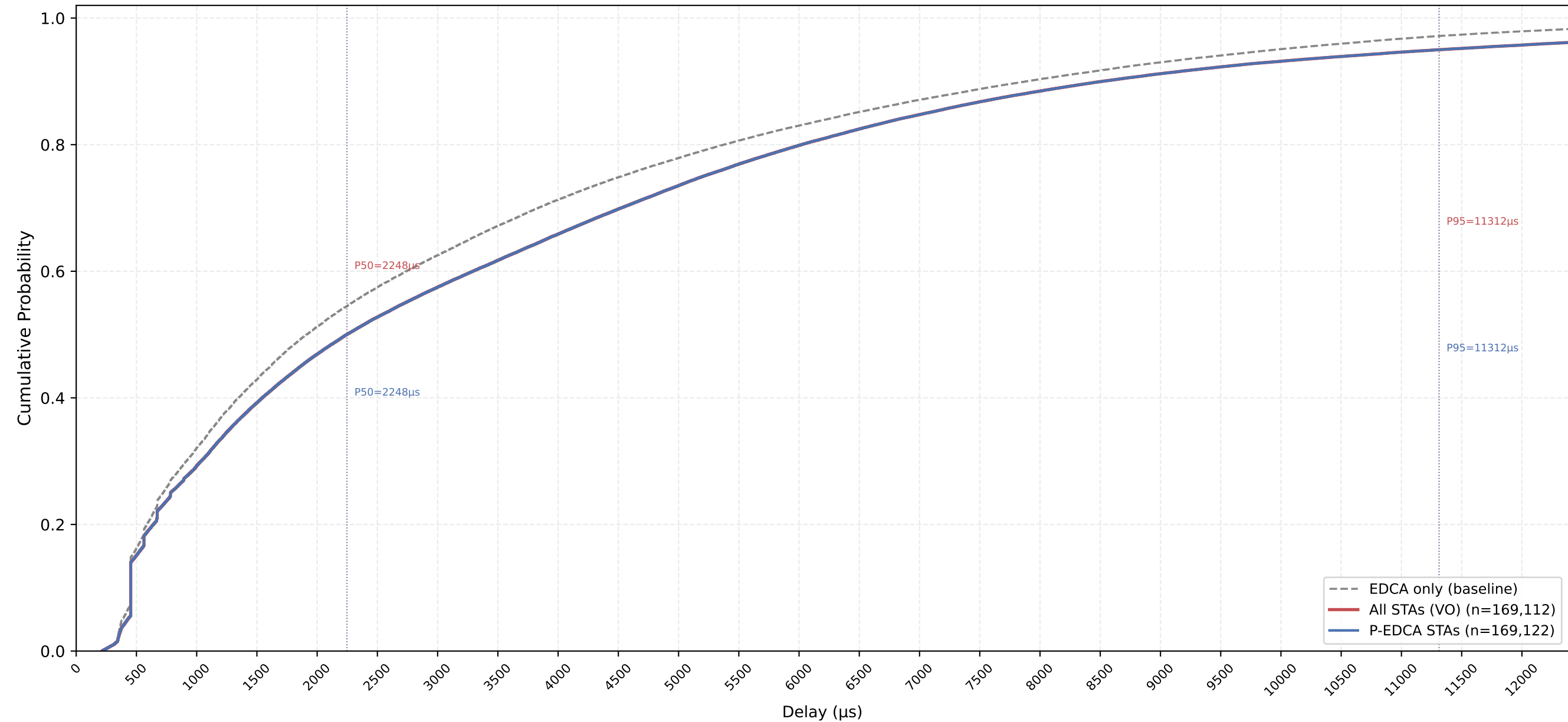
VO Delay CDF — P-EDCA / Legacy / All | CWds=1 × QSRC=3 × PSRC=2 nSta=30, nPedca=30/30, 1Mbps, avg of 10 runs
