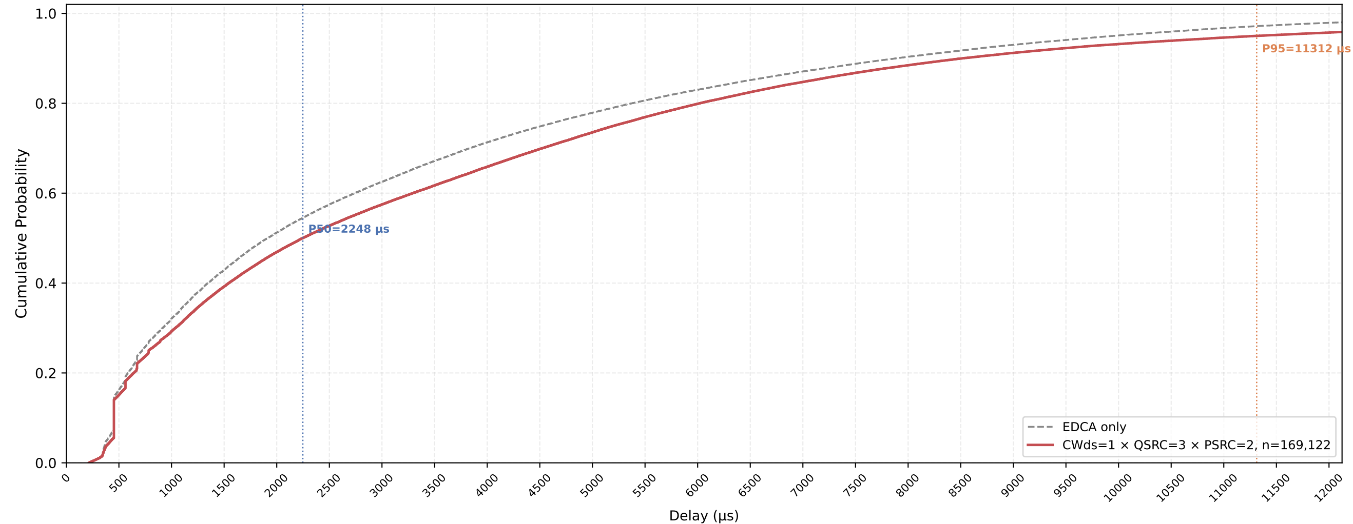
P-EDCA STA VO Delay CDF — CWds=1 × QSRC=3 × PSRC=2 nSta=30, nPedca=30, 1Mbps, avg of 10 runs
