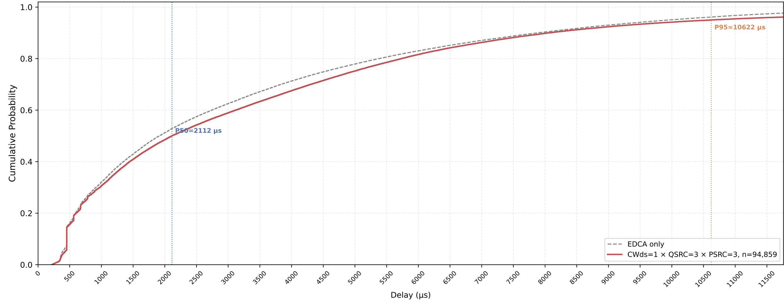
P-EDCA STA VO Delay CDF — CWds=1 × QSRC=3 × PSRC=3 nSta=30, nPedca=15, 1Mbps, avg of 10 runs
