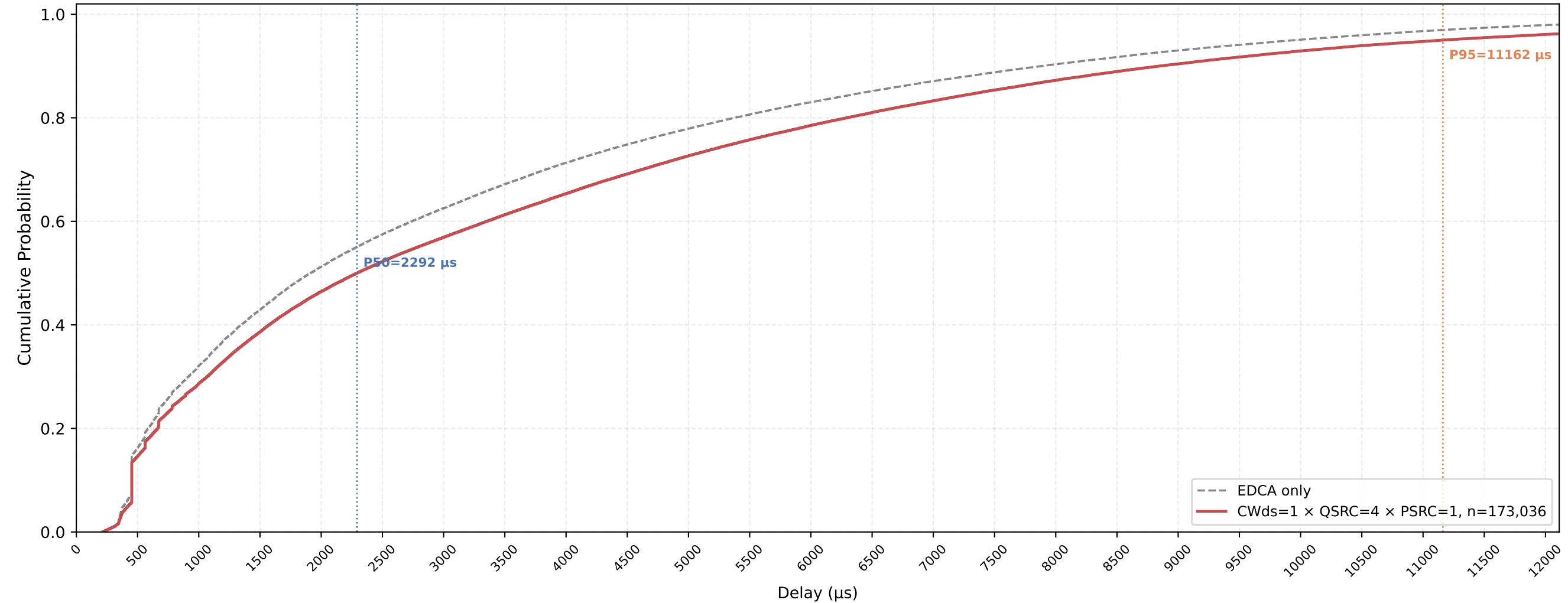
P-EDCA STA VO Delay CDF — CWds=1 × QSRC=4 × PSRC=1 nSta=30, nPedca=30, 1Mbps, avg of 10 runs
