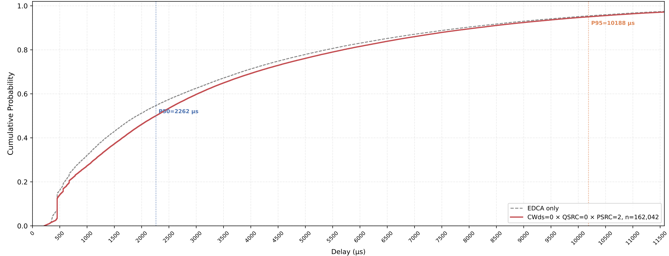
P-EDCA STA VO Delay CDF — CWds=0 × QSRC=0 × PSRC=2 nSta=30, nPedca=30, 1Mbps, avg of 10 runs
