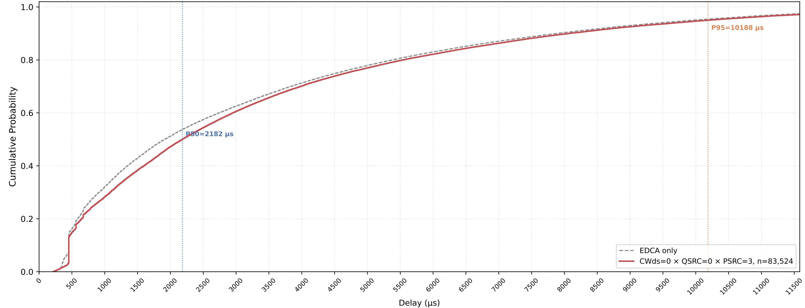
P-EDCA STA VO Delay CDF — CWds=0 × QSRC=0 × PSRC=3 nSta=30, nPedca=15, 1Mbps, avg of 10 runs
